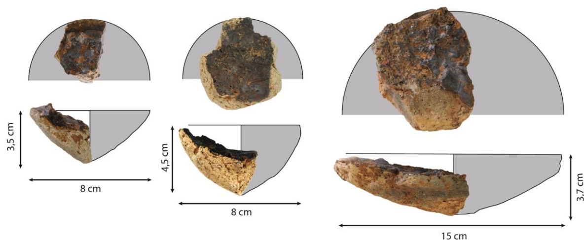
Figure 4 : Examples of archaeological crucibles from Vilabouly
