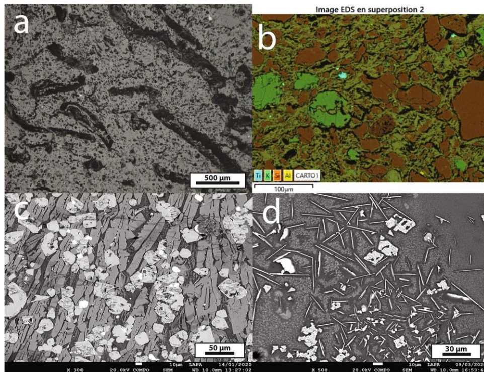
Figure 8 : a OM image of the crucible paste of sample PBL/ A15/4/1/6709/b with rice chaff voids; b SEM–EDS X-ray map (K \alpha ROIs) of the crucible paste of sample PBL/B17/2/1/3303/f zone containing potassium feldspars, quartz grains and rutile identified by their composition and habits; c SEM-BSE image with an example of fayalitic lattices in the interior of the crucible PBL/C14/2/3/7217; d SEMBSE image with an example of a vitreous copper-rich slag for the sample DF/1-A/4/131/a with delafossite needles
