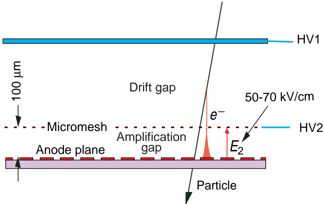
Figure 35.11: Schematic drawing of the Micromegas detector.
