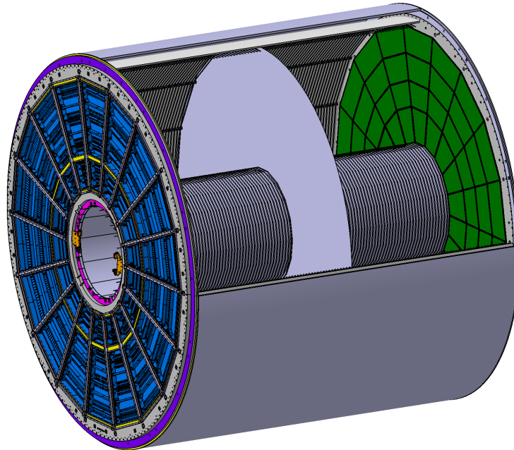
Figure 35.14: Schematic view of the ALICE TPC [168,169]. The drift volume with 5 m diameter is divided into two halves, each providing 2.5 m drift length. The amplification stage has recently been upgraded from wire planes to GEMs.
