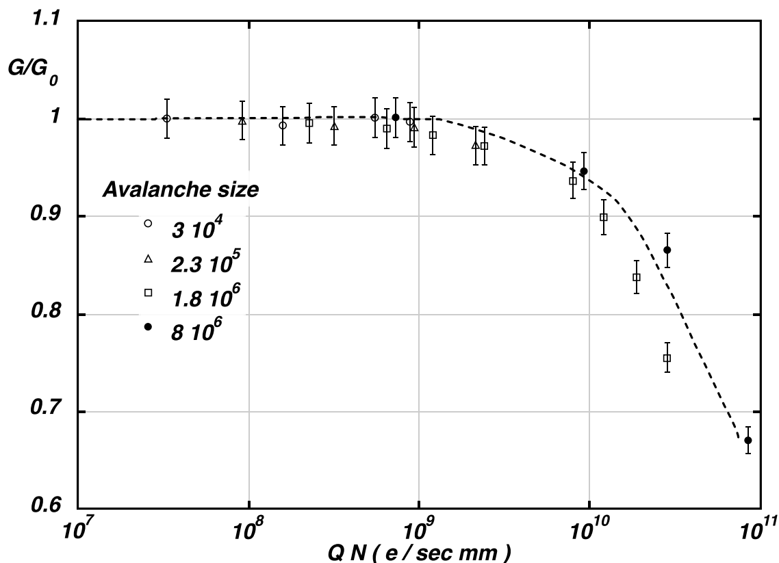
Figure 35.9: Charge rate dependence of normalized gas gain G/G_0 (relative to zero counting rate) in proportional thin-wire detectors [132]. Q is the total charge in single avalanche; N is the particle rate per wire length.
