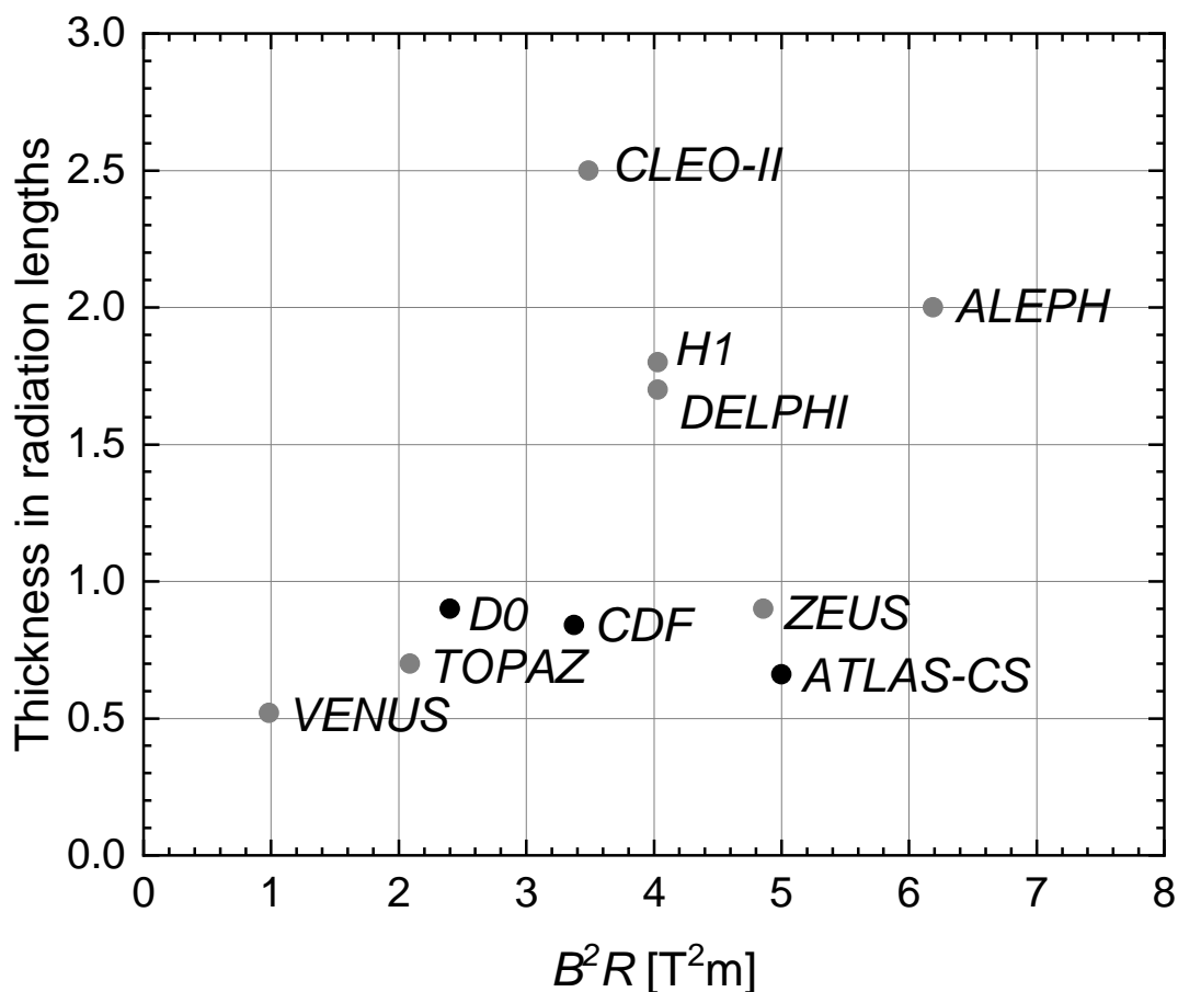
Figure 35.35: Magnet wall thickness in radiation length as a function of B^2R for various detector solenoids. Gray entries are for magnets no longer in use.
