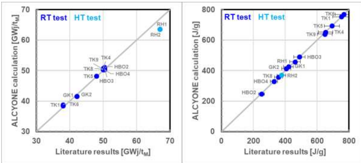
Fig 4. ALCYONE calculated versus literature values of (left) burnup and (right) peak enthalpy increase (symbols: dark blue for RT test, light blue for HT test)
