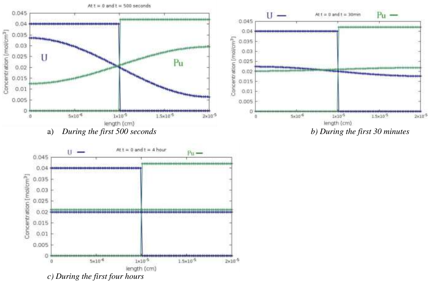
Figure 2 : Concentration profiles of U and Pu as a function of distance between the two half-couples of interdiffusion using Neumann boundary conditions
