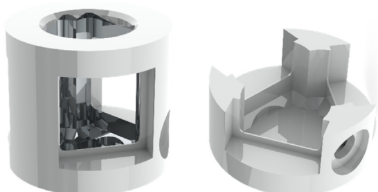
Fig. 6. 3D image of the optical chamber covered by reflective foil. The complex shape allows the light to be redirected towards the PMT active areas.
