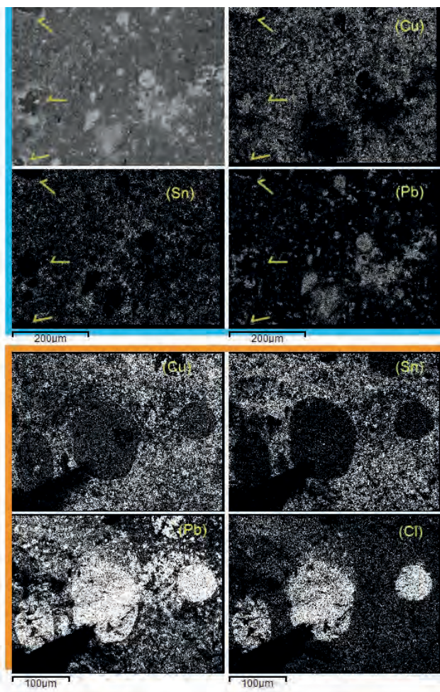
Figure 3 | 2053; SEM-EDX elemental mapping. Above: metal surface; arrows point the replacement of Pb globules with cuprite. Below: internal layer; Cl has interacted mostly with Pb globules that were detached from the metal surface during sampling.
