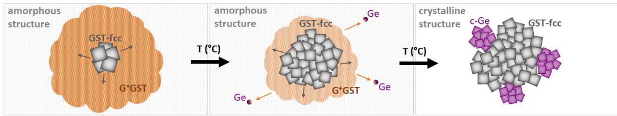
Fig. 9: Scheme representing the progress of GST225-fcc phase crystallization, disappearance of transient G^+GST phase with the expulsion of Ge atoms and following Ge phase crystallization with increasing annealing temperature.
