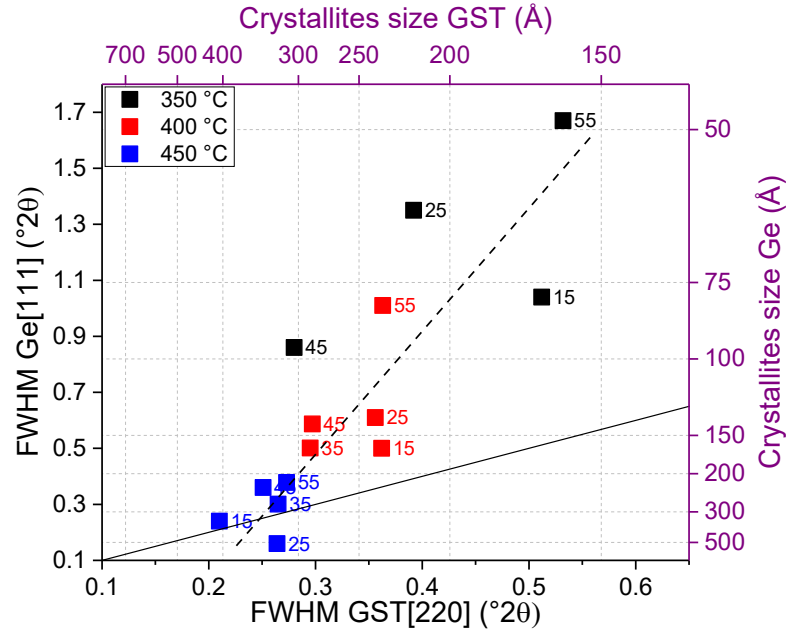
Fig. 7: Correlation of the FWHM and crystallites sizes for the GST 225 -fcc phase and Ge crystalline phases (dashed line). The values were taken from the GST[220] and Ge[111] peaks. The solid line represents the 1:1 ratio between the crystallites size of both phases.
