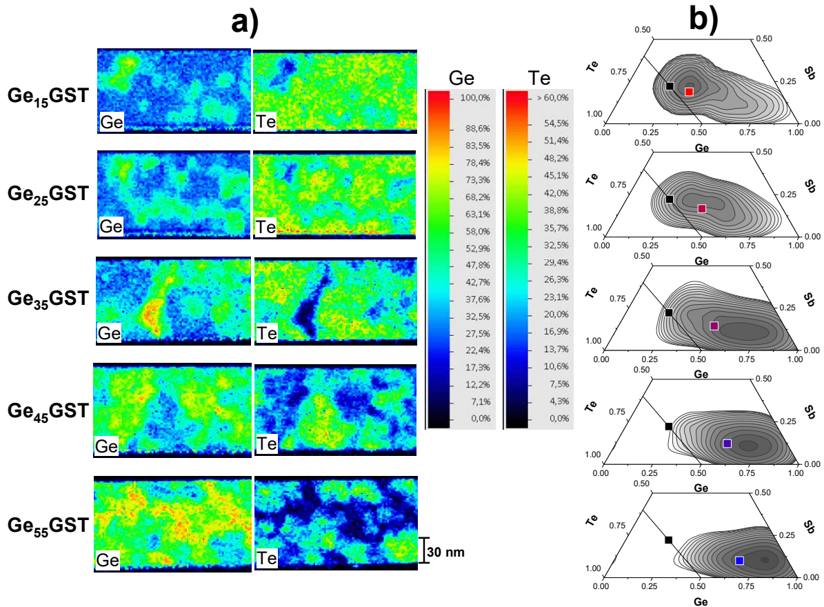
Fig. 10 : TEM-EDX analyses on Ge_xGST layers annealed at 400 °C. a) Ge and Te cartographies highlighting the elemental migration; b) Ge-Sb-Te ternary diagram showing the compositional distribution along the tie line
