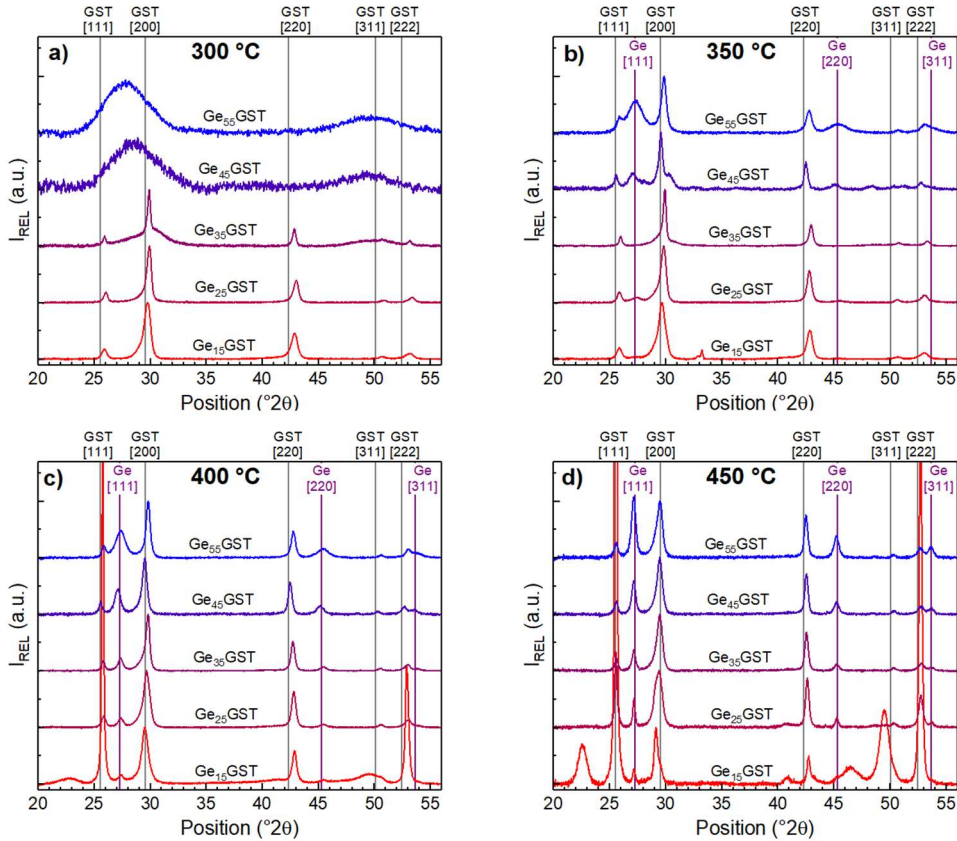
Fig. 6: XRD patterns of Ge x GST layers annealed at 300 °C (a), 350 °C (b), 400 °C (c), and 450 °C (d).
