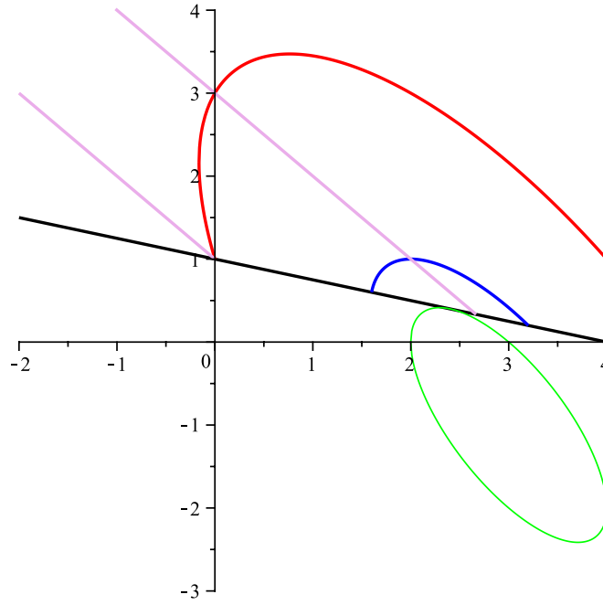
FIGURE 11. Domain lines in the (q, \eta_1) plane, for the \eta_2 = 4 - q case. The two purple straight lines have for equations, \eta_1 = 1 - q and \eta_1 = 3 - q . The green, blue and red ellipses have for respective equations X^2 + Y^2 = 1, 2, 10 , with X = q - 3, Y = \eta_1 + q - 2 , with same center located at (q, \eta_1) = (3, -1) .
