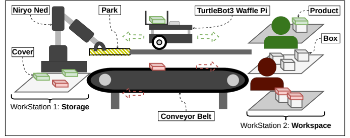
Fig. 2. Product Assembly Line for box manufacturing deployed in LocalSEA
