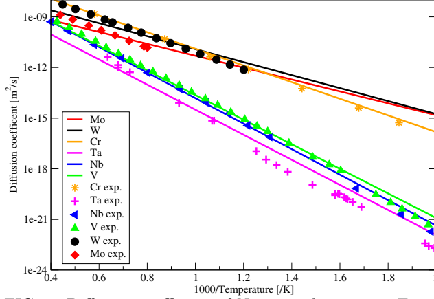
FIG. 5. Diffusion coefficient of N in metal matrices. Experiment data for Cr are reported in [39], Ta, Nb, and V in [40], W in [41], and Mo in [42]
