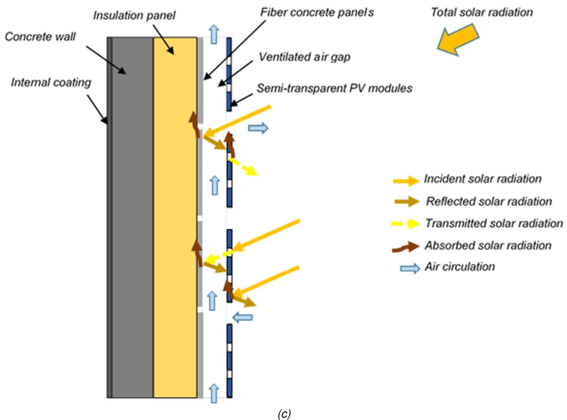
Figure 2: Schemes of the insulated fiber concrete panel (a) and photograph (b) of the CONIPHER BIPV panel and working principle on the solar facade vertical section considering expected air flow direction in the air gap and main solar radiation transmissions (with PV cells on blue zones and semi-transparent areas on white zones of PV modules) (c)
