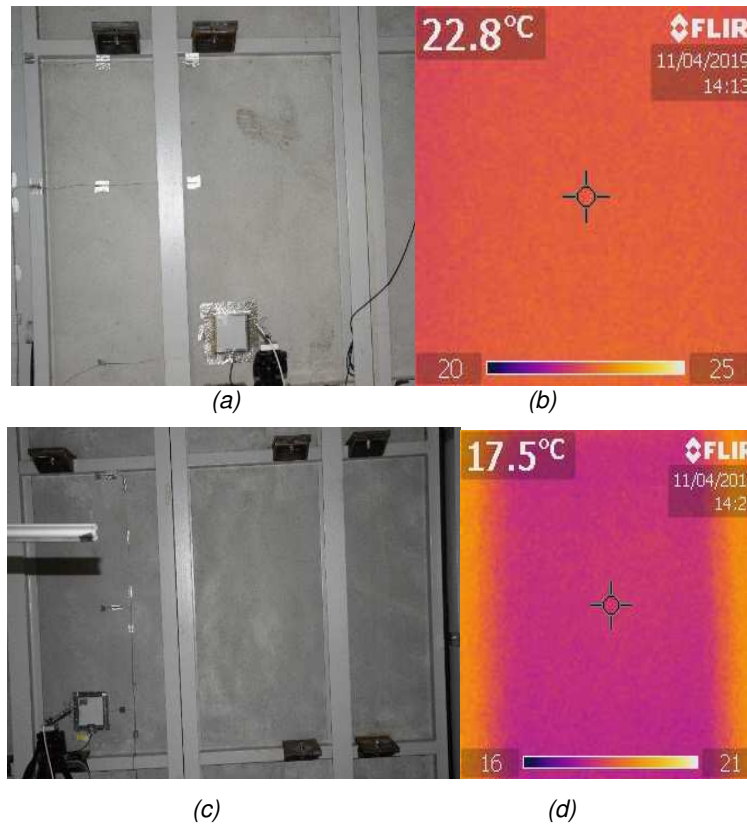
Figure 12: Photographs and thermal images of the internal coatings of the south-oriented facades of test cell 4 (a and b) and test cell 3 (c and d) from 2:12 pm to 2:21 pm on a day in April with low solar radiation.
