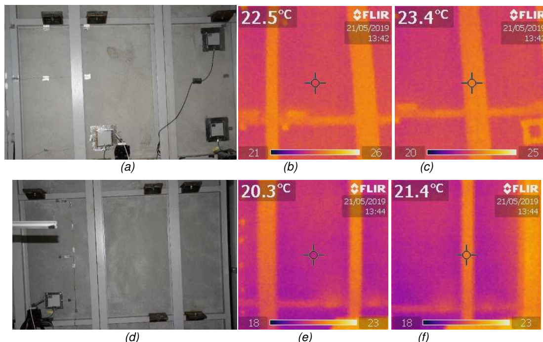
Figure 14: Photographs and thermal images of the internal coatings of the south-oriented facades of test cell 4 (a, b and c) and of test cell 3 (d, e and f) obtained with a thermal camera from 1:34 to 1:44 pm on a day in May with high solar radiation.
