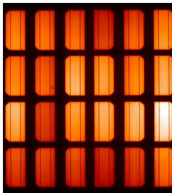
Figure 3: Electroluminescence image of a bifacial PV module.
