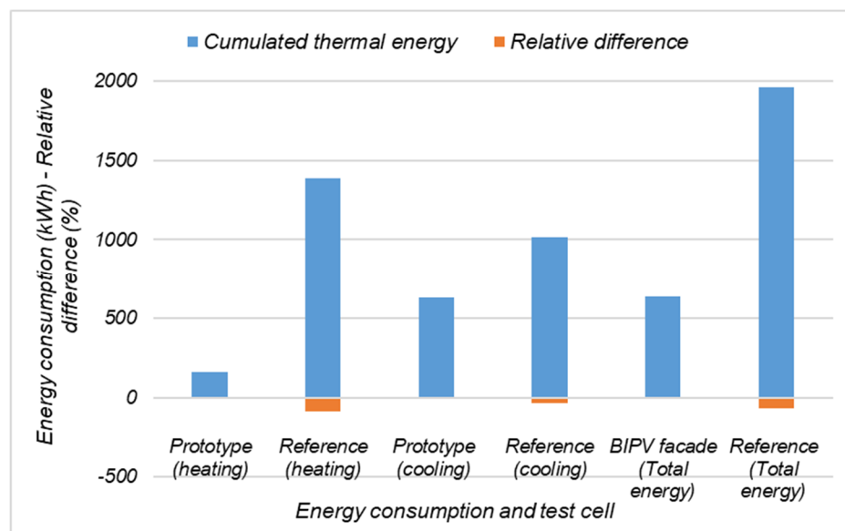
Figure 16: Cumulated values of the total energy consumption and energy consumptions for heating and cooling needed to maintain the setpoint temperature in the test cell 3 (reference) and in the test cell 4 (with the BIPV facade) (in kWh) and relative differences of energy consumption (in %) from December 2018 to December 2019.
