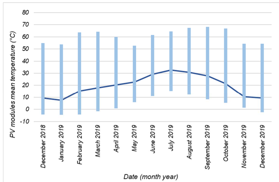
Figure 10: Monthly variations of the PV field mean temperature based on the PV modules 3 and 5 front glass temperatures and monthly average values (dark blue line) from December 2018 to December 2019.
