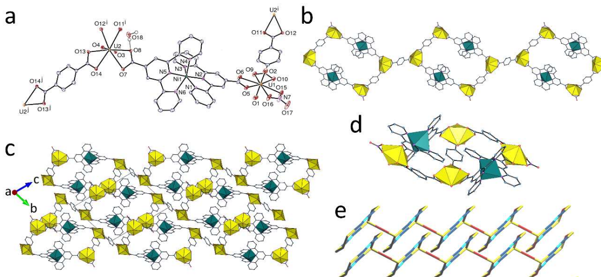
Figure 4. (a) View of compound 3 . Displacement ellipsoids are drawn at the 50% probability level. The acetonitrile molecule and carbon-bound hydrogen atoms are omitted, and the hydrogen bond to a water molecule is shown as a dashed line. Symmetry codes: i = 2 - x, 1 - y, 1 - z ; j = 1 - x, -y, -z . (b) View of the monoprotic coordination polymer with uranium coordination polyhedra yellow and those of nickel green. (c) Packing with chains viewed sideways. (d) chain viewed down its axis. (e) Simplified representation showing the arrangement of chains (view down [101] with [010] horizontal; uranium, yellow; nickel, light blue; \text{tpyc}^- ligands, dark blue; \text{bdc}^{2-} , red).
