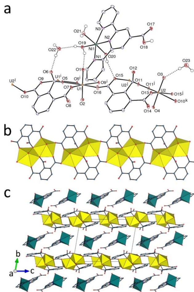
Figure 8. (a) View of compound 7. Displacement ellipsoids are drawn at the 50% probability level. Carbon-bound hydrogen atoms are omitted and hydrogen bonds are shown as dashed lines. Symmetry codes: i = 1 - x, -y, -z ; j = -x, -y, 1 - z ; k = x - 1, y, z + 1 ; l = x + 1, y, z - 1 . (b) View of the monoperiodic coordination polymer. (c) Packing with uranium coordination polyhedra yellow and those of nickel green.
