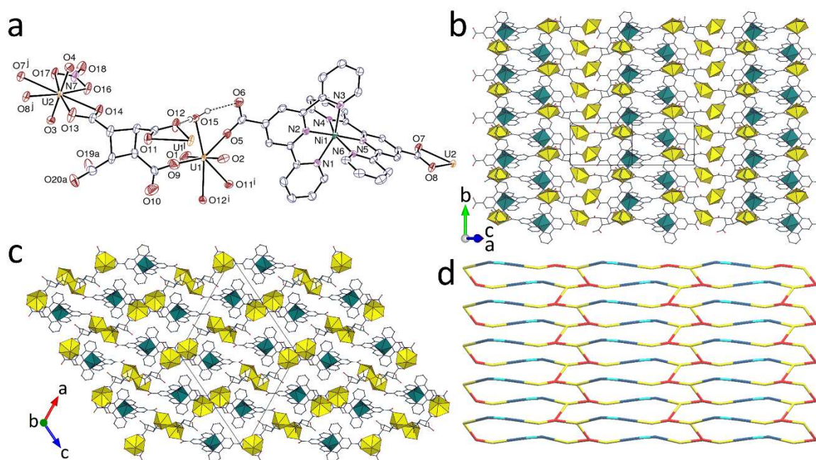
Figure 11. (a) View of compound 10 . Displacement ellipsoids are drawn at the 50% probability level. Carbon-bound hydrogen atoms are omitted and hydrogen bonds are shown as dashed lines. Only one position of the disordered atoms is shown. Symmetry codes: i = 1 - x, y + 1/2, 3/2 - z ; j = x + 1, y, z + 1 ; k = x - 1, y, z - 1 ; l = 1 - x, y - 1/2, 3/2 - z . (b) View of the diperiodic network with uranium coordination polyhedra yellow and those of nickel green. (c) Packing with layers viewed edge-on. (d) Simplified view of the network (uranium, yellow; nickel, light blue; tpyc - ligands, dark blue; cbtcH 3- ligands, red).
