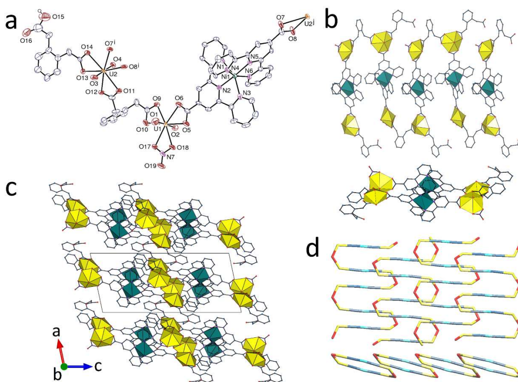
Figure 6. (a) View of compound 5 . Displacement ellipsoids are drawn at the 50% probability level. The solvent molecule and carbon-bound hydrogen atoms are omitted. Symmetry codes: i = 1 - x, y + 1/2, 1/2 - z ; j = 1 - x, y - 1/2, 1/2 - z . (b) Two views of the zigzag monoperiodic coordination polymer face-on or end-on, with uranium coordination polyhedra yellow and those of nickel green. (c) Packing with chains viewed end-on. (d) Simplified views showing the arrangement of chains, face-on or end-on (uranium, yellow; nickel, light blue; \text{tpyc}^- ligands, dark blue; bridging 1,2\text{-pda}^{2-} ligands, red).
