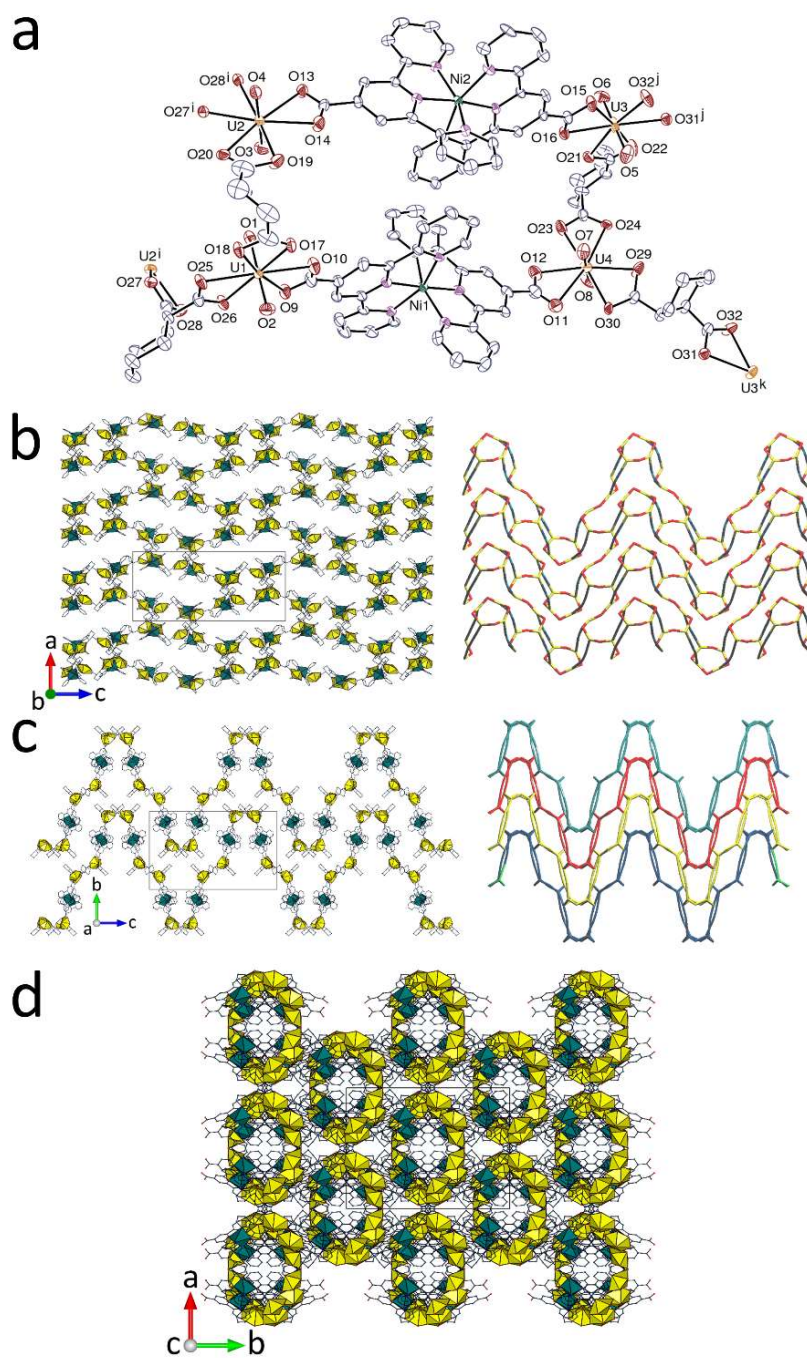
Figure 13. (a) View of compound 12 . Displacement ellipsoids are drawn at the 30% probability level and hydrogen atoms are omitted. Only one position of the disordered atoms is shown. Symmetry codes: i = 1 - x, y, 3/2 - z ; j = x - 1/2, 1/2 - y, 1 - z ; k = x + 1/2, 1/2 - y, 1 - z . (b) View of the dimeric network with uranium coordination polyhedra yellow and those of nickel green (left), and slightly rotated simplified view (right; uranium, yellow; nickel, light blue; tpyc^- ligands, dark blue; t-R-1,2-chdc^{2-} ligands, red). (c) Two layers viewed edge-on, with one intermediate layer omitted for clarity (left), and simplified view of four interlocked layers (right). (d) Another view of the packing with layers viewed edge-on.
