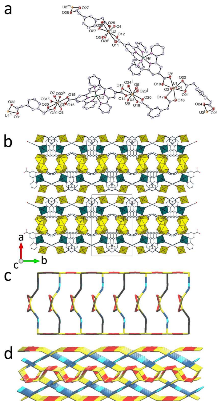
Figure 14. (a) View of compound 13. Displacement ellipsoids are drawn at the 30% probability level. Solvent molecules and hydrogen atoms are omitted. Only one position of the disordered atoms is shown. Symmetry codes: i = x, -y, z - 1/2 ; j = x, y - 1, z ; k = x, -y - 1, z + 1/2 ; l = x, y + 1, z ; m = x, -y, z + 1/2 ; n = x, -y - 1, z - 1/2 . (b) Packing with two layers viewed edge-on. Uranium coordination polyhedra are yellow and those of nickel green. (c) and (d) Simplified views of the diperiodic assembly down [010] with [001] horizontal, and down a direction slightly rotated from that in b (uranium, yellow; nickel, light blue; tpyc - ligands, dark blue; 1,3-pda 2- ligands, red).
