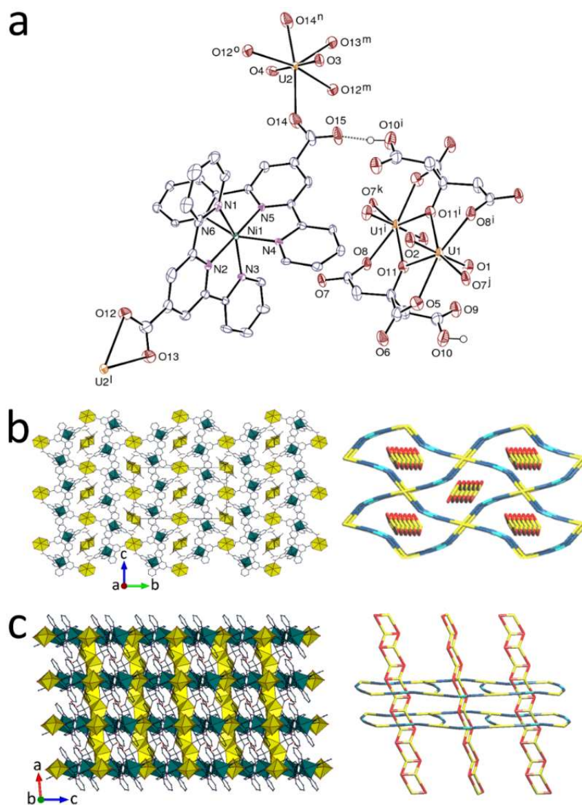
Figure 9. (a) View of compound 8 . Displacement ellipsoids are drawn at the 50% probability level. Carbon-bound hydrogen atoms are omitted and the hydrogen bond is shown as a dashed line. Only one position of the disordered atoms is shown. Symmetry codes: i = 1 - x, 1 - y, 1 - z ; j = x + 1, y, z ; k = -x, 1 - y, 1 - z ; l = -x, y - 1/2, 3/2 - z ; m = -x, y + 1/2, 3/2 - z ; n = -x, 1 - y, 2 - z ; o = x, 1/2 - y, z + 1/2 . (b) Dipericodic network viewed side-on and monopericodic chains viewed end-on, with uranium coordination polyhedra yellow and those of nickel green (left), and slightly rotated simplified view (right; uranium, yellow; nickel, light blue; tpyc - ligands, dark blue; citH 3- ligands, red). (c) Packing with sheets viewed edge-on (left), and simplified view of the two assembled coordination polymers (right).
