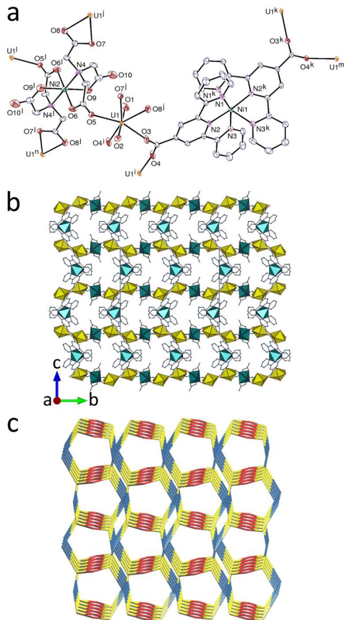
Figure 15. (a) View of compound 14. Displacement ellipsoids are drawn at the 50% probability level and hydrogen atoms are omitted. Symmetry codes: i = -x, 1 - y, 1 - z ; j = 1/2 - x, 3/2 - y, 1 - z ; k = 1 - x, y, 1/2 - z ; l = -x - 1/2, 3/2 - y, 1 - z ; m = x + 1, 1 - y, z - 1/2 ; n = x - 1, y, z . (b) View of the three-periodic framework with uranium coordination polyhedra yellow and those of nickel green. (c) Nodal representation of the framework, slightly rotated with respect to the orientation in b (uranium, yellow; Ni(tpyc) 2 nodes, dark blue; Ni(nta) 2 4+ nodes, red).
