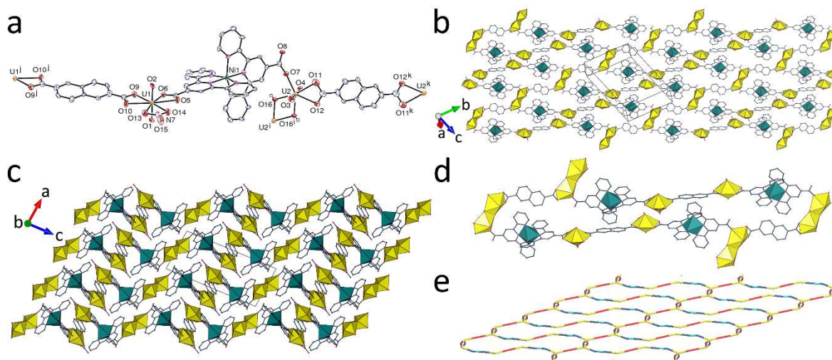
Figure 12. (a) View of compound 11 . Displacement ellipsoids are drawn at the 50% probability level and carbon-bound hydrogen atoms are omitted. Symmetry codes: i = 1 - x, 1 - y, -z ; j = 2 - x, 3 - y, 1 - z ; k = 1 - x, -y, -z . (b) View of the diperiodic network with uranium coordination polyhedra yellow and those of nickel green. (c) Packing with layers viewed edge-on. (d) View of one 14-nuclear ring. (e) Simplified view of the network (uranium, yellow; nickel, light blue; \text{tpyc}^- ligands, dark blue; 2,6- \text{ndc}^{2-} ligands, red; hydroxide groups, orange).
