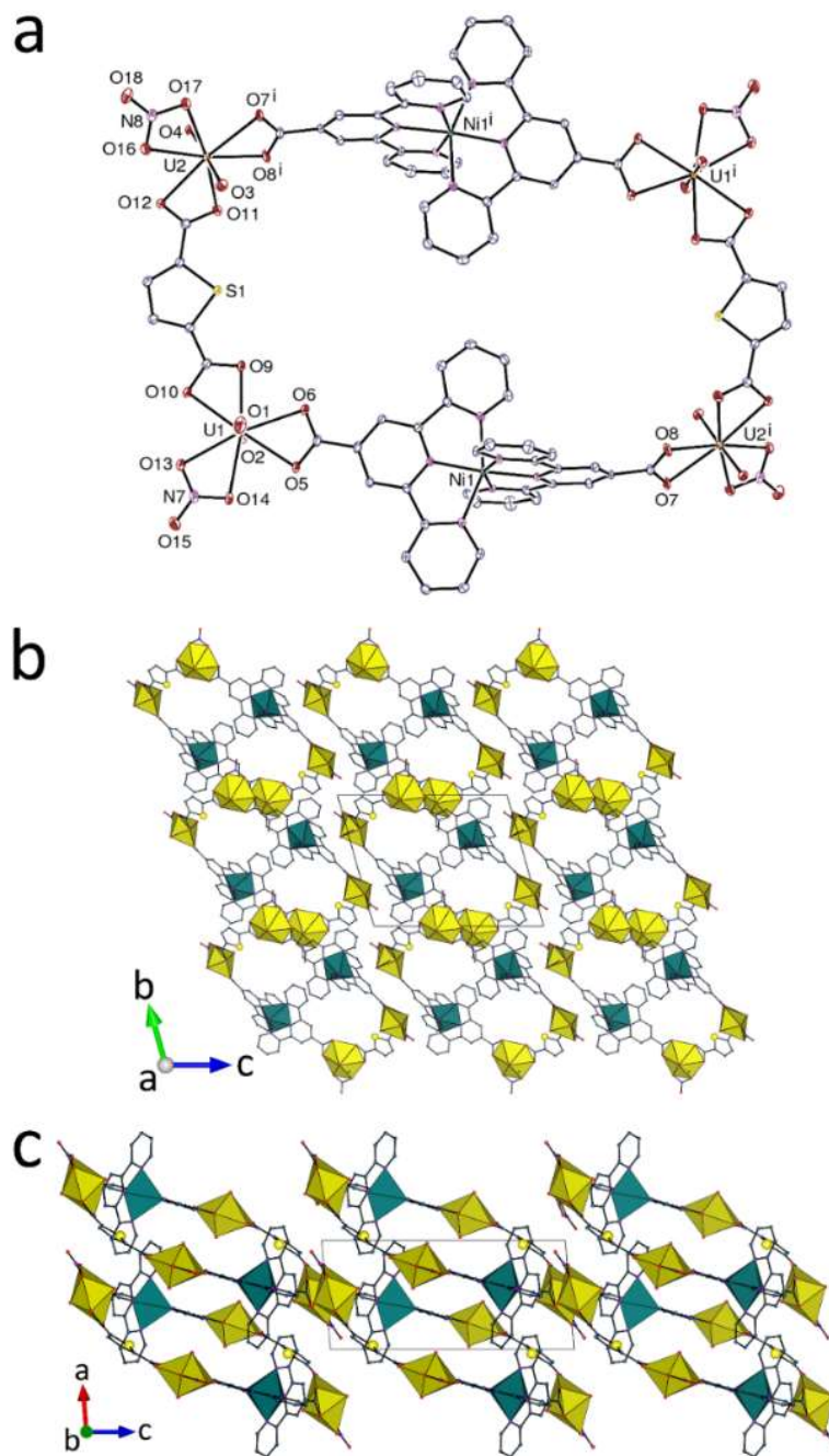
Figure 2. (a) View of compound 2 . Displacement ellipsoids are drawn at the 50% probability level and hydrogen atoms are omitted. Symmetry code: i = 2 - x, 1 - y, 1 - z . (b, c) Two views of the packing with uranium coordination polyhedra yellow and those of nickel green.
