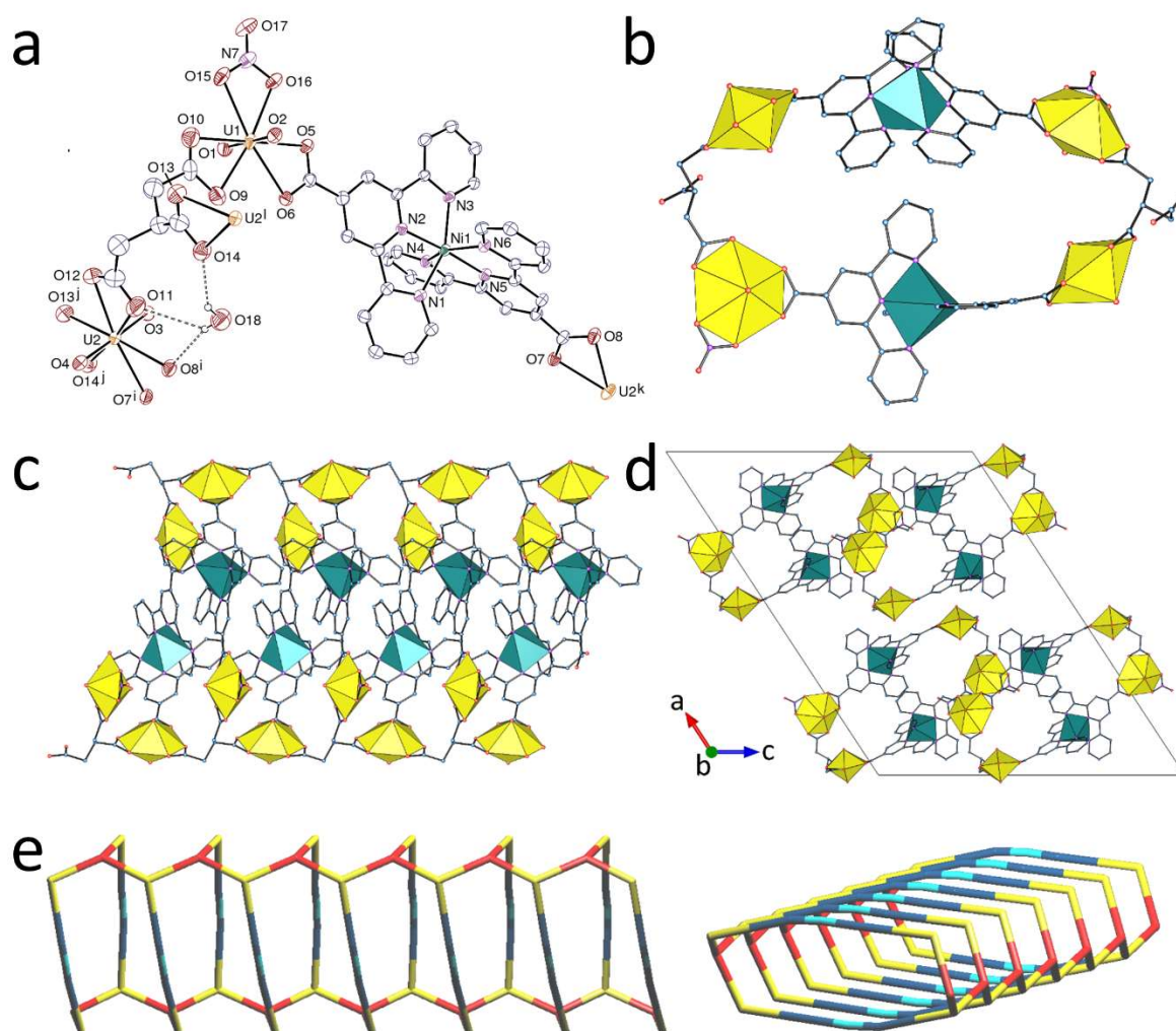
Figure 5. (a) View of compound 4 . Displacement ellipsoids are drawn at the 30% probability level. The acetonitrile molecules and carbon-bound hydrogen atoms are omitted, and hydrogen bonds are shown as dashed lines. Symmetry codes: i = 1/2 - x, y - 1/2, 1/2 - z ; j = x, y - 1, z ; k = 1/2 - x, y + 1/2, 1/2 - z ; l = x, y + 1, z . (b) View of the U_4Ni_2 ring with uranium coordination polyhedra yellow and those of nickel green. (c) View of the monoperiodic coordination polymer. (d) Packing viewed down the nanotube axis. (e) Two views of the simplified representation of the nanotube (uranium, yellow; nickel, light blue; tpyc^- ligands, dark blue; tca^{3-} ligands, red).
