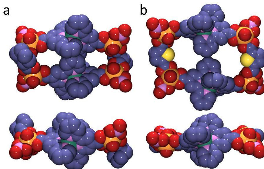
Figure 3. Space-filling representations of the rings in complexes 1 (a) and 2 (b) viewed down two orthogonal directions (uranium, orange; nickel, green; sulfur, yellow; oxygen, red; nitrogen, purple; carbon, blue; hydrogen atoms are omitted).
