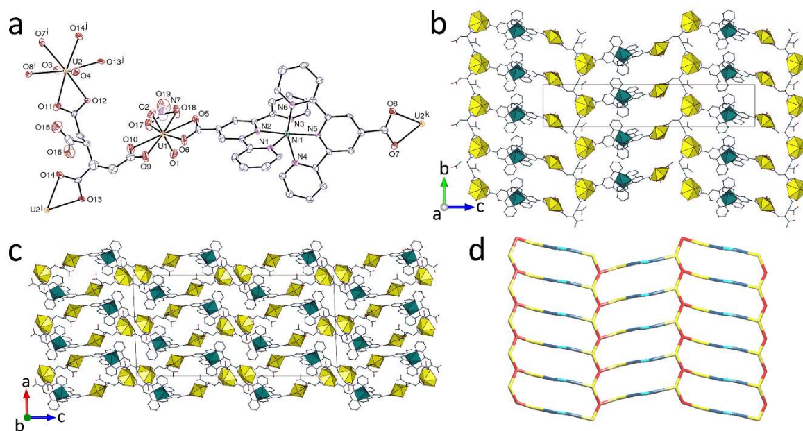
Figure 10. (a) View of compound 9 . Displacement ellipsoids are drawn at the 50% probability level and hydrogen atoms are omitted. Symmetry codes: i = x, 2 - y, z - 1/2 ; j = x, y + 1, z ; k = x, 2 - y, z + 1/2 ; l = x, y - 1, z . (b) View of the diperiodic network with uranium coordination polyhedra yellow and those of nickel green. (c) Packing with layers viewed edge-on. (d) Simplified view of the network (uranium, yellow; nickel, light blue; \text{tpyc}^- ligands, dark blue; \text{btcH}^{3-} ligands, red).
