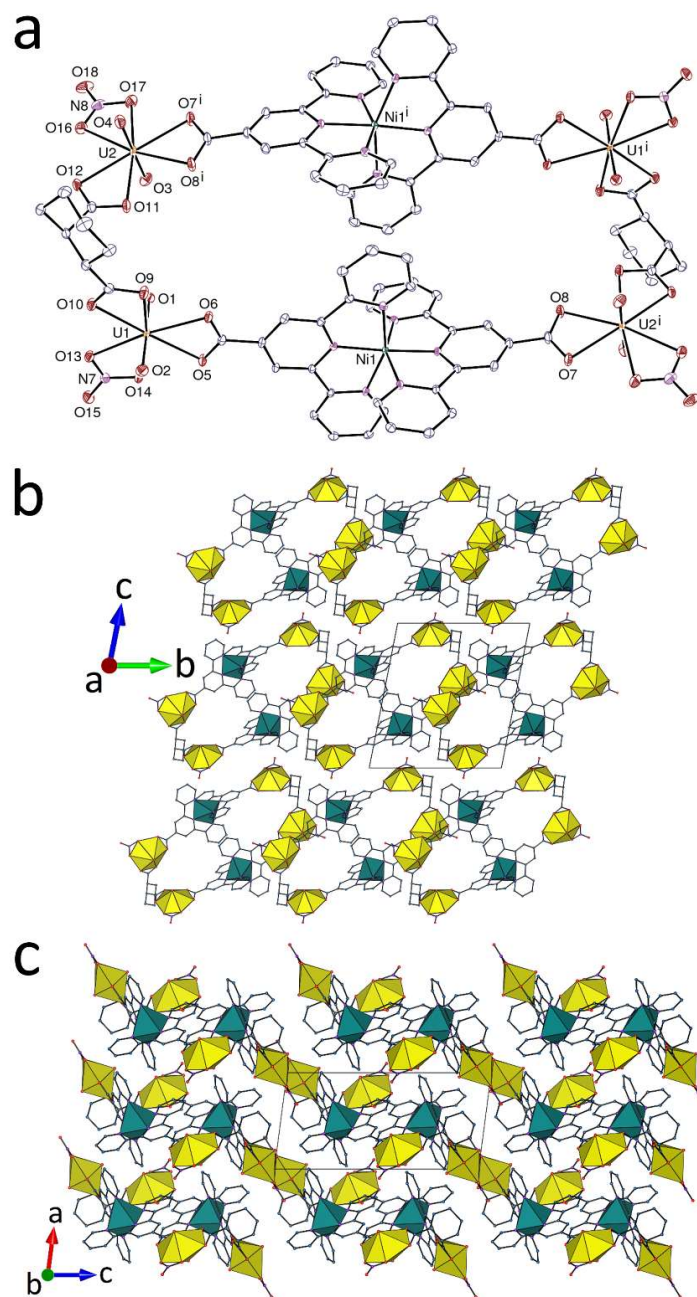
Figure 1. (a) View of compound 1. Displacement ellipsoids are drawn at the 50% probability level. Solvent molecules and hydrogen atoms are omitted. Symmetry code: i = 1 - x, 2 - y, 1 - z . (b, c) Two views of the packing with uranium coordination polyhedra yellow and those of nickel green.
