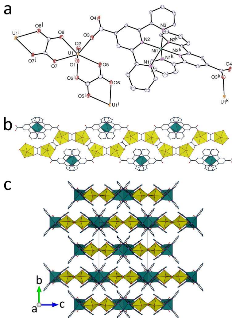
Figure 7. (a) View of compound 6 . Displacement ellipsoids are drawn at the 50% probability level and hydrogen atoms are omitted. Symmetry codes: i = 1 - x, 1 - y, -z ; j = 3/2 - x, 1 - y, z ; k = 1/2 - x, 1 - y, z . (b) View of the monoperiodic coordination polymer with uranium coordination polyhedra yellow and those of nickel green. (c) Packing with chains viewed end-on.
