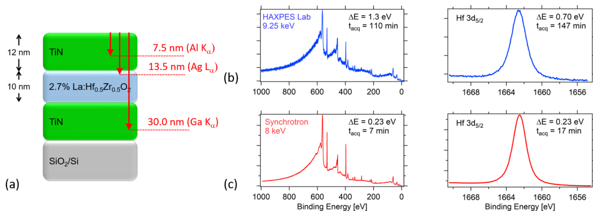
Fig. 2. (color online). (a) Schematic of 12 nm TiN/10 nm La : HfZrO 2 /12 nm TiN/SiO 2 /Si test sample. The approximate probing depths of Hf 3d electrons excited by Al K \alpha , Ag L \alpha and Ga K \alpha are shown by the red arrows. The graphs show the survey (left) and Hf 3d 5/2 core level (right) spectra obtained using (b) HAXPES Lab and (c) synchrotron radiation. For each spectrum, the energy resolution \Delta E and the total acquisition time t_{\text{acq}} are indicated.
