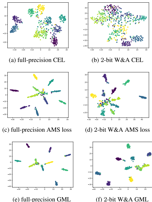
Figure 1. Dimension reduction with t-sne algorithm representing the input features of the linear classifier from CIFAR10 test data. The corresponding top-1 test accuracies are reported in Tab. 1. t-sne performed over 1000 iterations and a perplexity of 30.
