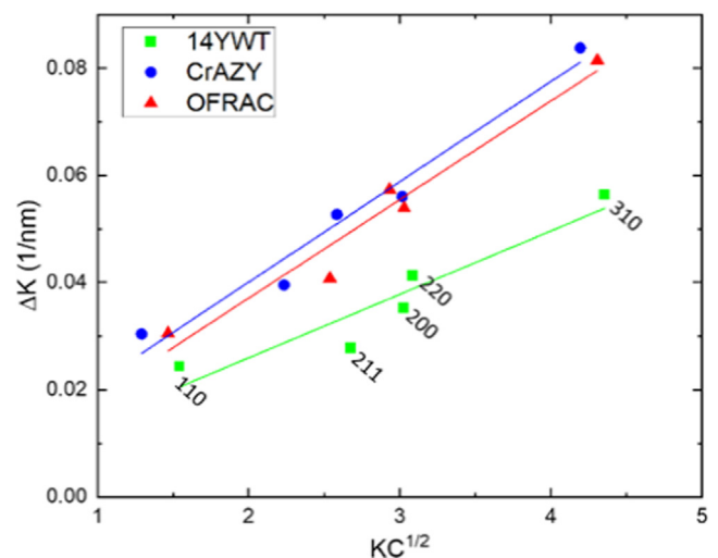
Fig. 8. Linear slope fitting of the mod. Williamson-Hall plot for the three materials.
