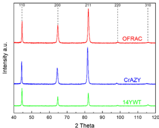
Fig. 7. Intensity XRD profiles in arbitrary units of the three materials are plotted against 2 Theta with a y-offset for comparison reasons. Corresponding hkl values for each peak are shown along the top of the figure.
