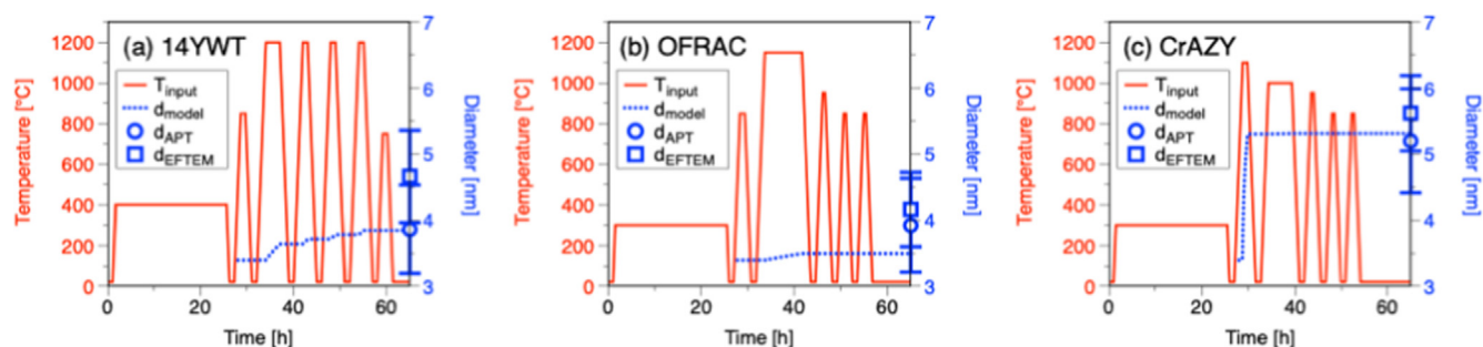
Fig. 14. Comparison between measured (EFTEM/APT) precipitate sizes and that estimated using state-of-the-art coarsening models. The solid red profile represents the temperature history of each tube as the original mechanically alloyed powder was subjected to degassing, extrusion, and intermediate annealing treatments during the pilgering process, and the blue line presents the model precipitate diameter at each time step. (For interpretation of the references to color in this figure legend, the reader is referred to the web version of this article.)
