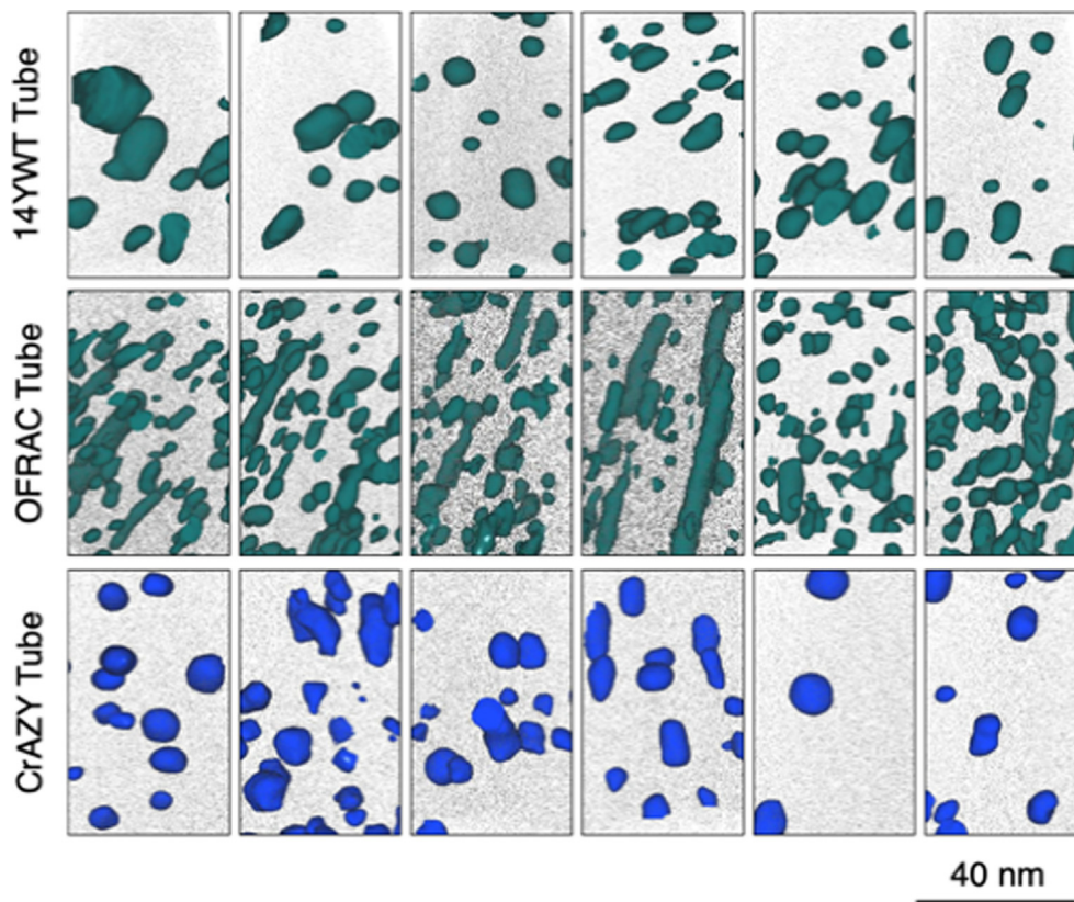
Fig. 9. APT volumes measuring 40 \times 40 \times 65 \text{ nm}^3 show the precipitate dispersions in each tube. Green isoconcentration surfaces highlight regions enriched in at least 1.5% (Y + Ti + O), and blue surfaces represent regions with 1.5% enrichment of (Y + Al + O). In each image, 0.1% of background Fe atoms are also presented as black dots. (For interpretation of the references to color in this figure legend, the reader is referred to the web version of this article.)
