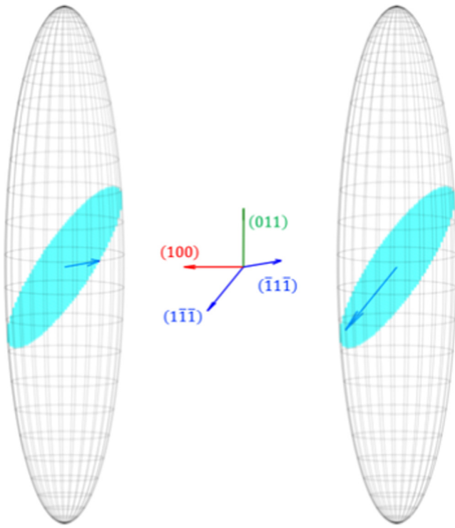
Fig. 3. Three-dimensional views of a spheroidal grain of aspect ratio 5:1 with major axis oriented parallel to [011] with resolved slip along (110)[111] and (110)[\bar{1}11] .
