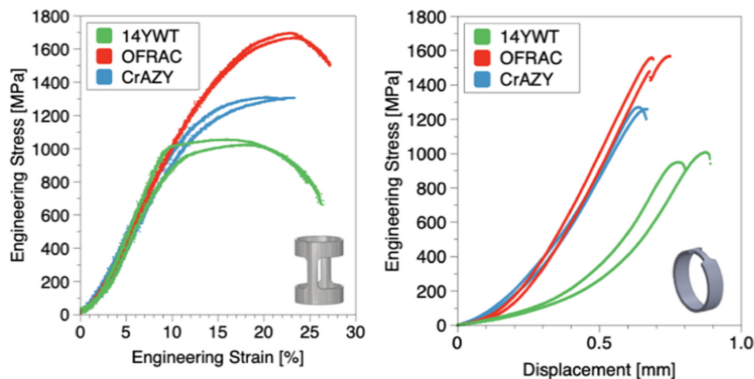
Fig. 11. Room temperature tensile response of axial (left) and ring-pull (right) specimens from each ODS tube. For axially loaded specimens, the engineering stress is plotted as a function of engineering strain, and for ring-pull specimens the stress is plotted as a function of crosshead displacement.
