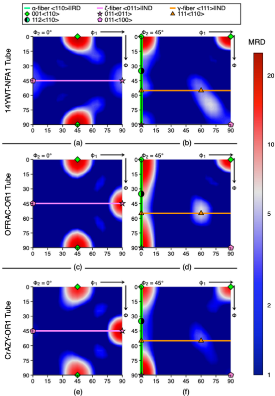
Fig. 5. ODF contour plots for each thin-walled tube computed from EBSD methods. All plots use Euler angle representation and highlight two characteristic slices at \phi_2 = 0^\circ and 45^\circ where major rolling texture components for BCC materials are visible. All plots are normalized to the same color bar in units of multiples of random density.
