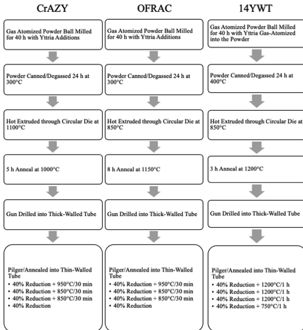
Fig. 1. Process diagrams for thin-walled ODS FeCr(Al) tubes produced via pilgering.
