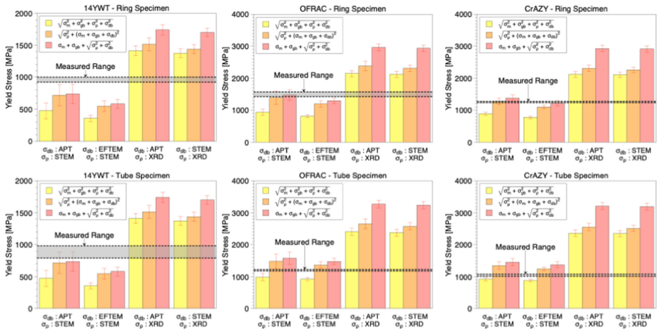
Fig. 13. Experimentally measured vs. estimated yield strengths for ring-pull and axial tube tests for 14YWT, OFRAC, and CrAZY tubes. The results are categorized as a function of the superposition approach and the method used to estimate input parameters for dislocation and precipitate characteristics. Error bars represent one standard deviation from the mean computed using a Monte Carlo error propagation approach.
