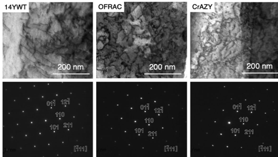
Fig. 6. Typical BF STEM images of dislocation networks in each ODS FeCr(Al) alloy tube. All micrographs are imaged along the \langle 111 \rangle -zone axis, as confirmed by the accompanying indexed diffraction patterns.
