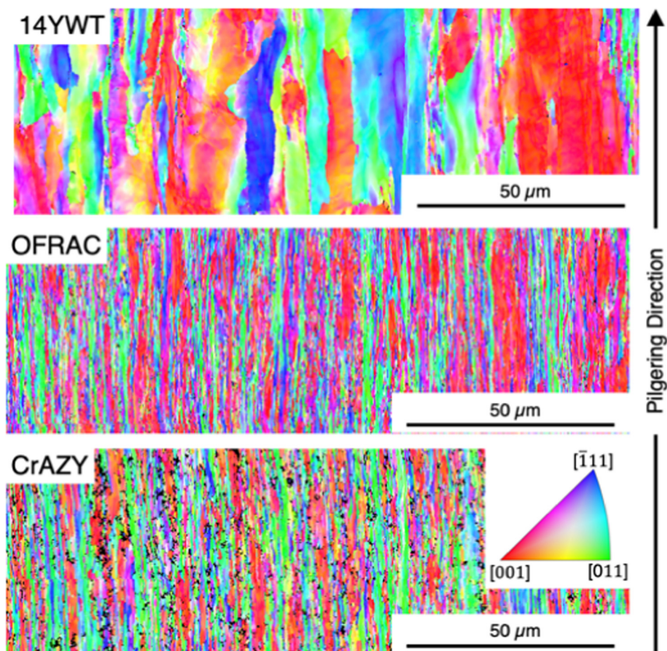
Fig. 4. EBSD IPF maps showing differences in grain size, morphology, and orientation. The tube axis (pilgering direction) is oriented vertically in all images.
