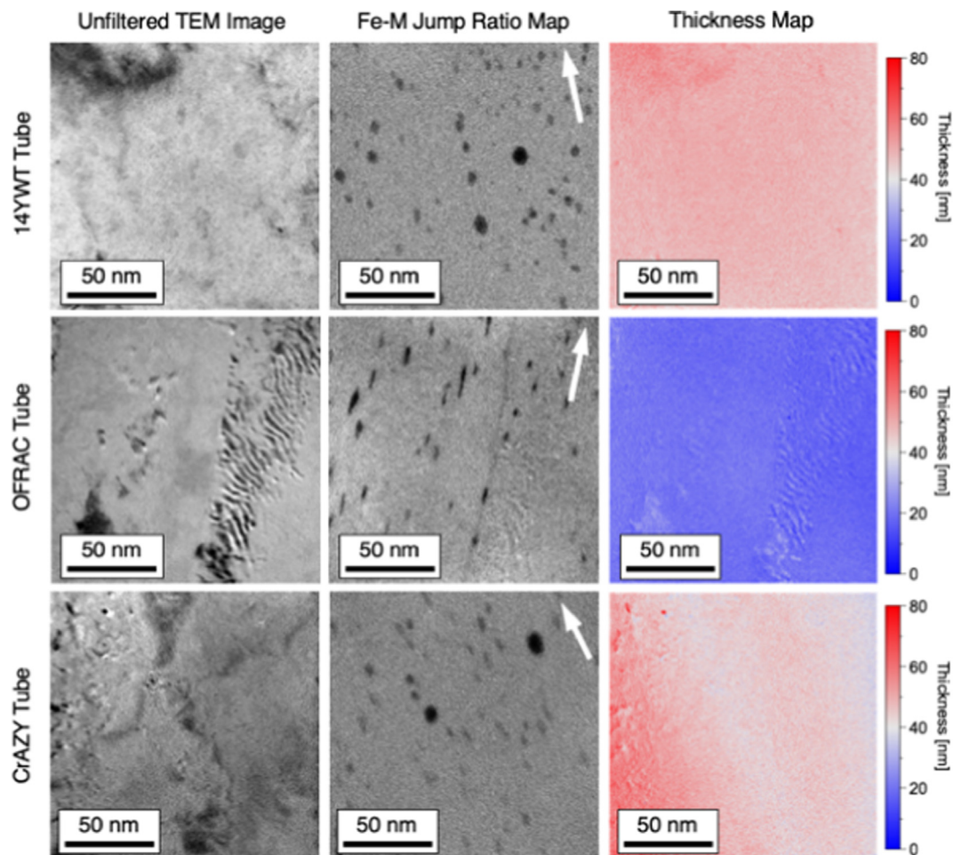
Fig. 10. Representative EFTEM maps for particle size and density calculations. The unfiltered TEM image of the region of interest is shown on the left, while the middle image is the jump ratio map for the Fe M-edge of the electron energy loss spectroscopy (EELS) spectrum. In the Fe-M jump ratio map, darker areas indicate a lack of Fe, while brighter regions indicate Fe enrichment. On the right, thickness maps and histograms are provided to convert precipitate areal density to number density.
