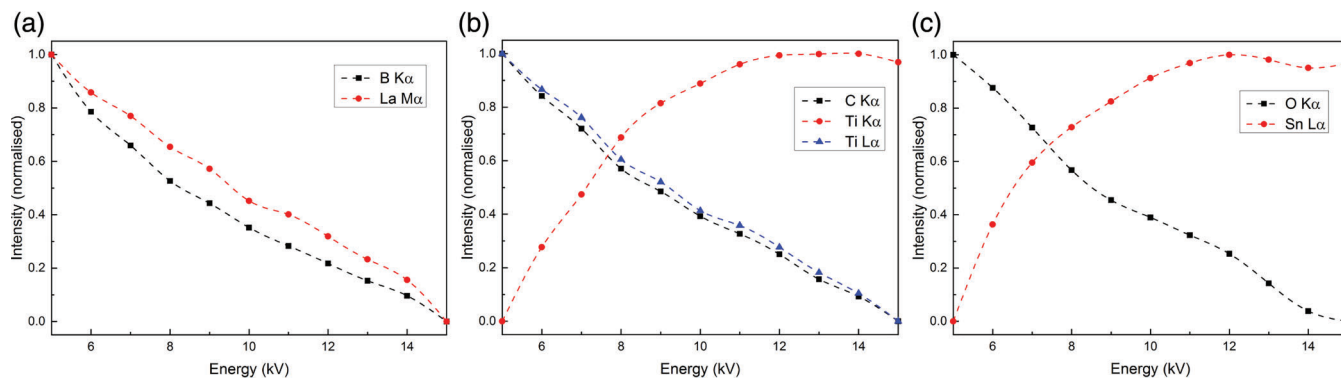
FIGURE 2 Normalised intensity of the characteristic X-rays as a function of the accelerating voltage applied to the microanalyser for the materials (a) \text{LaB}_6 , (b) \text{TiC} and (c) \text{SnO}_2 . The characteristic intensity depends on the ionisation cross section, the material's fluorescence yield and its absorption coefficient. Several Monte Carlo simulations are performed for every point and the statistical uncertainties are negligible compared to the large uncertainties in the database values used in the simulation software.
