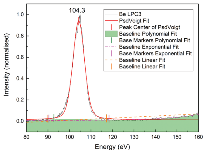
FIGURE 6 Pseudo-Voigt fit of the characteristic Be K\alpha peak with the three different background descriptions: The base markers define the integration area for net intensity and P/B ratios.
