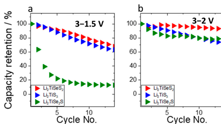
Figure 6. Capacity retention (%) of \text{Li}_2\text{TiS}_3 , \text{Li}_2\text{TiSeS}_2 , and \text{Li}_2\text{TiSe}_2\text{S} cells cycled at a rate of C/10 in different cycling windows: (a) 3–1.5 V and (b) 3–2.0 V vs. \text{Li}^+/\text{Li} .
