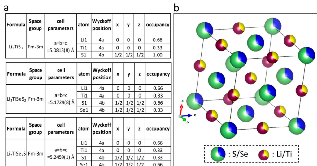
Figure 2. (a) Refined parameters of \text{Li}_2\text{TiSe}_x\text{S}_{3-x} ( 0 \leq x \leq 2 ) materials and (b) \text{Li}_2\text{TiSeS}_2 structure.
