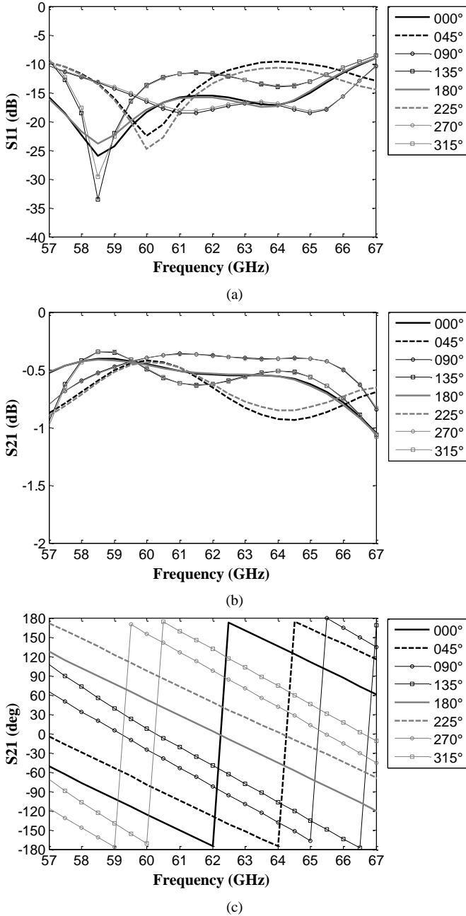
Fig. 3. 3-bit unit-cell simulated frequency response computed under normal incidence. (a) Amplitude of the reflection coefficient, (b) amplitude of the transmission coefficient, and (c) transmission phase.
