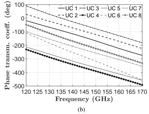
Fig. 3. (a) Amplitude and (b) phase of the transmission coefficients of the cells, simulated under normal incidence in an infinite periodic environment.
