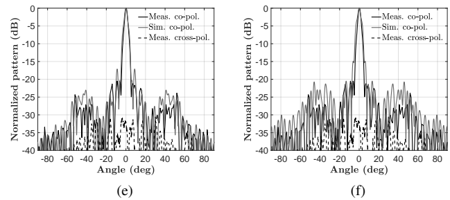
Fig. 8. Simulated and measured radiation patterns of the broadside lens at: (a) 130 GHz, H-plane; (b) 130 GHz, E-plane; (c) 145 GHz, H-plane; (d) 145 GHz, E-plane; (e) 160 GHz, H-plane; (f) 160 GHz, E-plane.
