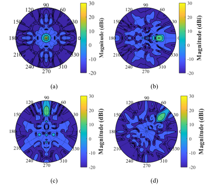
Fig. 9. Theoretical 2-D gain radiation patterns (Ludwig 3 co-polarization component) of the 2-bit steerable transmitarray achieved at 29 GHz when the nominal array layout without faulty unit-cells is considered. (a) Broadside, (b) (\theta_0, \phi_0) = (40^\circ, 0^\circ) , (c) (\theta_0, \phi_0) = (60^\circ, 90^\circ) , and (d) (\theta_0, \phi_0) = (60^\circ, 45^\circ) .
