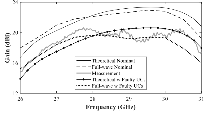
Fig. 5. Theoretical, simulated, and measured broadside gain of the TA prototype as a function of frequency.
