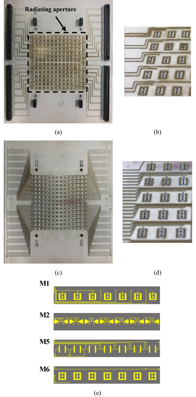
Fig. 3. Photographs of the realized electronically steerable transmitarray, (a)-(b) receiving and (c)-(d) transmitting layers with p-i-n diodes. (e) Schematic view of the bias network on one line of the 7 \times 7 subarray.
