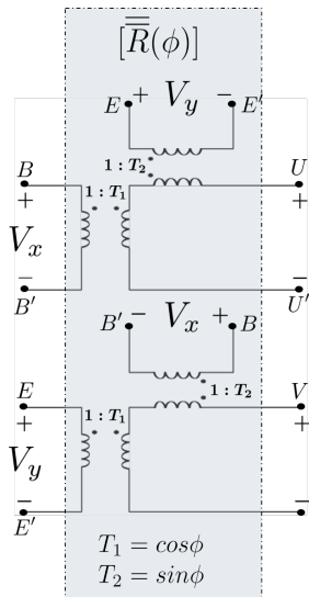
Fig. 3: Equivalent circuit of the rotation matrix, describing the relationship between the electric field components in the two coordinate systems. Ideal transformers are considered for the angle of rotation. The transpose rotation matrix is modelled by a similar network.
