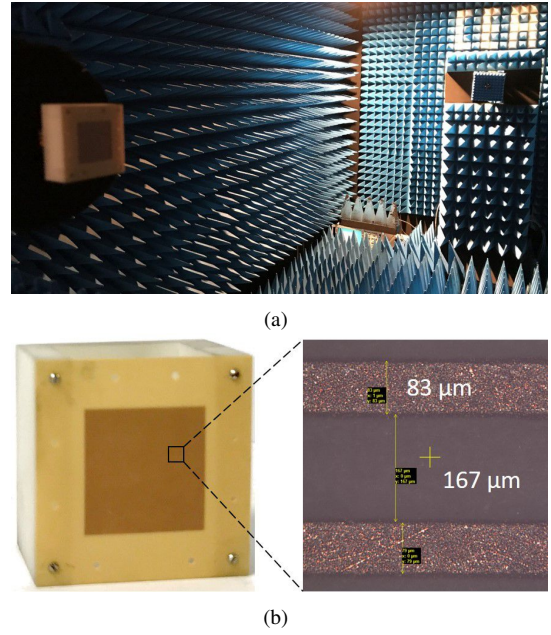
Fig. 9: (a) Measurement setup in the anechoic chamber and (b) view of the fabricated antenna prototype.
