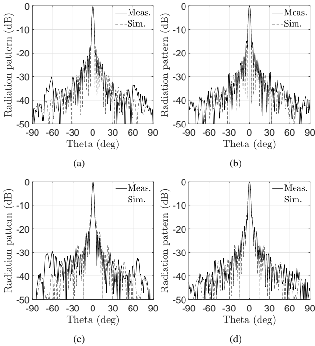
Fig. 11: Simulated and measured radiation pattern of the TA. (a) H-plane@280GHz, (b) E-plane@280GHz, (c) H-plane@300GHz and (d) E-plane@300GHz.
