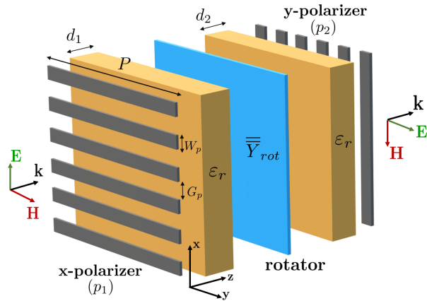
Fig. 1: Exploded view of the proposed unit-cell with P periodicity, which is the same along the x - and y -axis. The rotator (blue color) is generically modelled as a two-dimensional sheet impedance described by a 2 \times 2 admittance matrix. The polarization grids (grey color) are orthogonally oriented. The layers are interleaved by two dielectric spacers (orange color) of the same permittivity, \epsilon_r .
