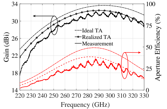
Fig. 10: Simulated and measured gain and aperture efficiency of the TA antenna prototype. The results are compared to an antenna comprising a perfect lens, considering the same focal source and focal distance.
