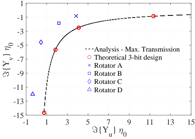
Fig. 6: Results of the synthesis procedure of the 3-bit TA at 300 GHz. By solving the expression (5) for maximum transmission, the dashed curve is derived. Assuming a 3-bit phase quantization, only four admittance pairs are needed (red circles), due to symmetry. The final results of the four rotators of Fig. 7 are depicted with blue symbols.
