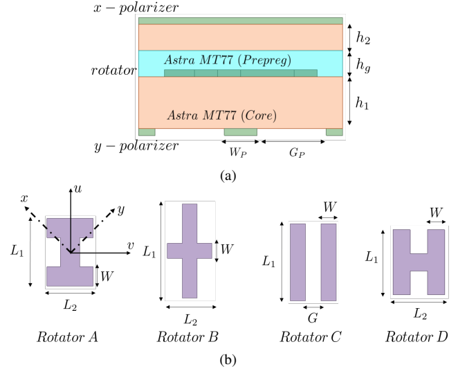
Fig. 7: (a) Stack-up of the unit-cells. (b) Rotator designs for the proposed 3-bit TA, in the (u, v) reference system (see Fig. 2). By mirroring each rotator with respect to the x -axis, the remaining four unit-cells are designed.
