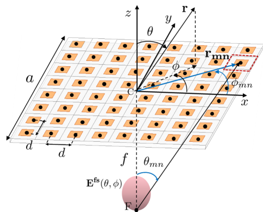
Fig. 1. Geometry of a transmitarray antenna and main parameters of the proposed model.
