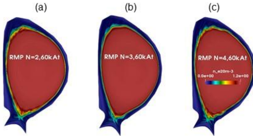
Fig.20. Electron density distribution in 15MA scenario with RMPs at maximum coils current 60kAt and RMP harmonic N=2 (a), N=3 (b) and N=4 (c) respectively. The common color bar is presented in (c). In each case the time of modelling corresponds to maximum time in Fig.17-18.
