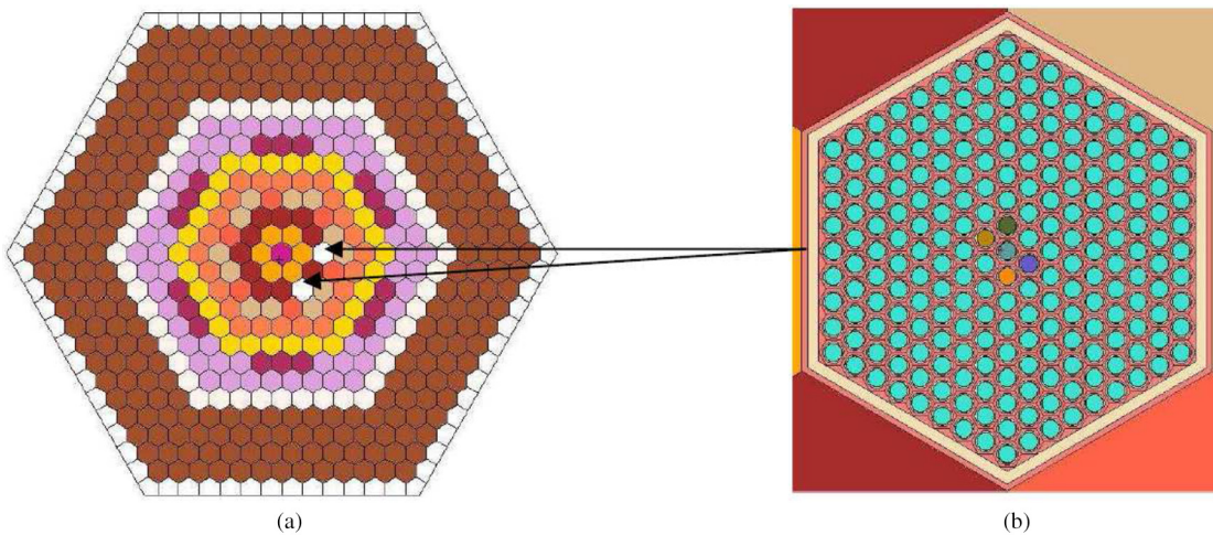
Fig. 8. Radial cross-sectional view of the TRAPU experiment. (a) Radial configuration during TRAPU experiment. (b) Subassembly containing irradiated samples.
