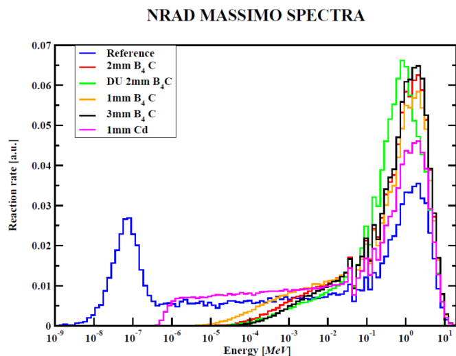
Fig. 21. Different spectra corresponding to different filters in MASSIMO experimental campaign.
