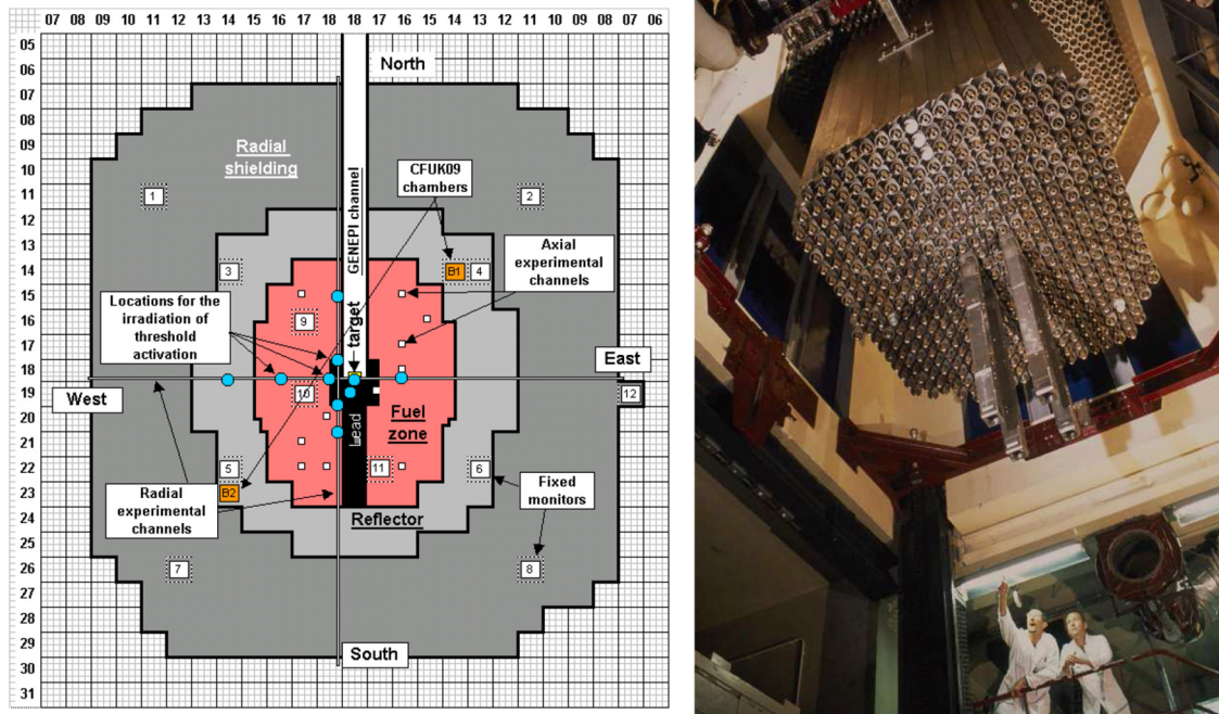
Fig. 12. The MUSE-4 Program: radical critical configuration (left), and actual MASURCA configuration (right: one can observe the GENEPI accelerator channel entering the core on the upper-left part).
