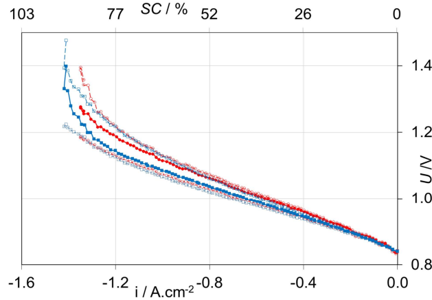
Figure 2: Initial iV curves in SOEC mode at 800°C for five ref cell stacks respectively 100 cm 2 of active area, red curves, and 196 cm 2 of active area, blue curves. Total flow rate of 12 NmL min -1 cm -2 of 90/10 vol.% H 2 O/H 2 mix is provided to the fuel electrode, air on the other side. Minimum, median and maximum cell voltages are represented by short dotted lines, full lines and long dotted lines respectively. Steam conversion is reported by secondary abscissa axis on top of the graph.
