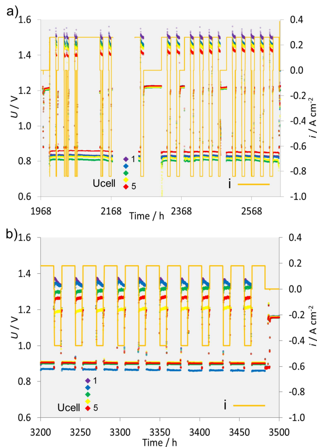
Figure 1: Daily switching tests for: a) Ref cell and b) G2 5-cell stacks, performed at 700°C. During 16h SOFC steps, stacks were fed with dry pure H 2 flow rate of 3 NmL min -1 cm -2 on fuel side and 5.4 NmL min -1 cm -2 on air side. For 8h SOEC steps stacks were fed with 90/10 vol.% H 2 O/H 2 mix at total flow rate 12 NmL min -1 cm -2 on fuel side and dry air on air side to ensure required differential pressure between gas compartments.
