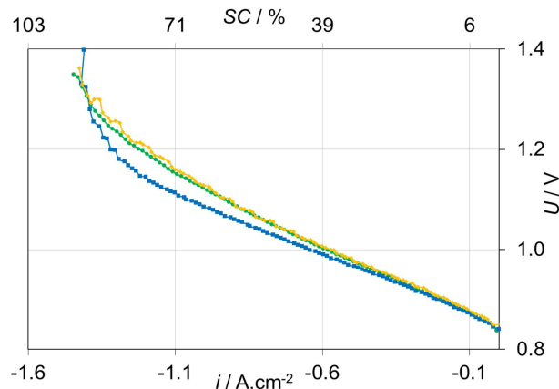
Figure 3: Initial iV curves in SOEC mode at 800°C for ref cells stacks, respectively 25 cells of 100 cm 2 active area : green circle dots, five cells of 196 cm 2 active area: blue square dots and 25 cells of 196 cm 2 active area : yellow diamond dots. Total flow rate of 12 NmL min -1 cm -2 of 90/10 vol.% H 2 O/H 2 mix is provided to the fuel electrode, air on the other side; median cell voltage is reported for each stack; steam conversion is reported by secondary abscissa axis top of the graph.
