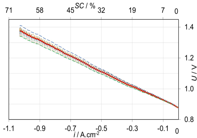
Figure 5: Cell voltage typical scattering recorded for a stack operated in SOEC providing 90/10 vol.% H 2 O/H 2 mix to the fuel electrode at 700°C. Cells voltage data are plotted with circle marks, the associated median cell voltage is plotted as a red continuous line, two dotted lines derived from median voltage curve highlight cell voltage scattering remains within \pm 7\% .
