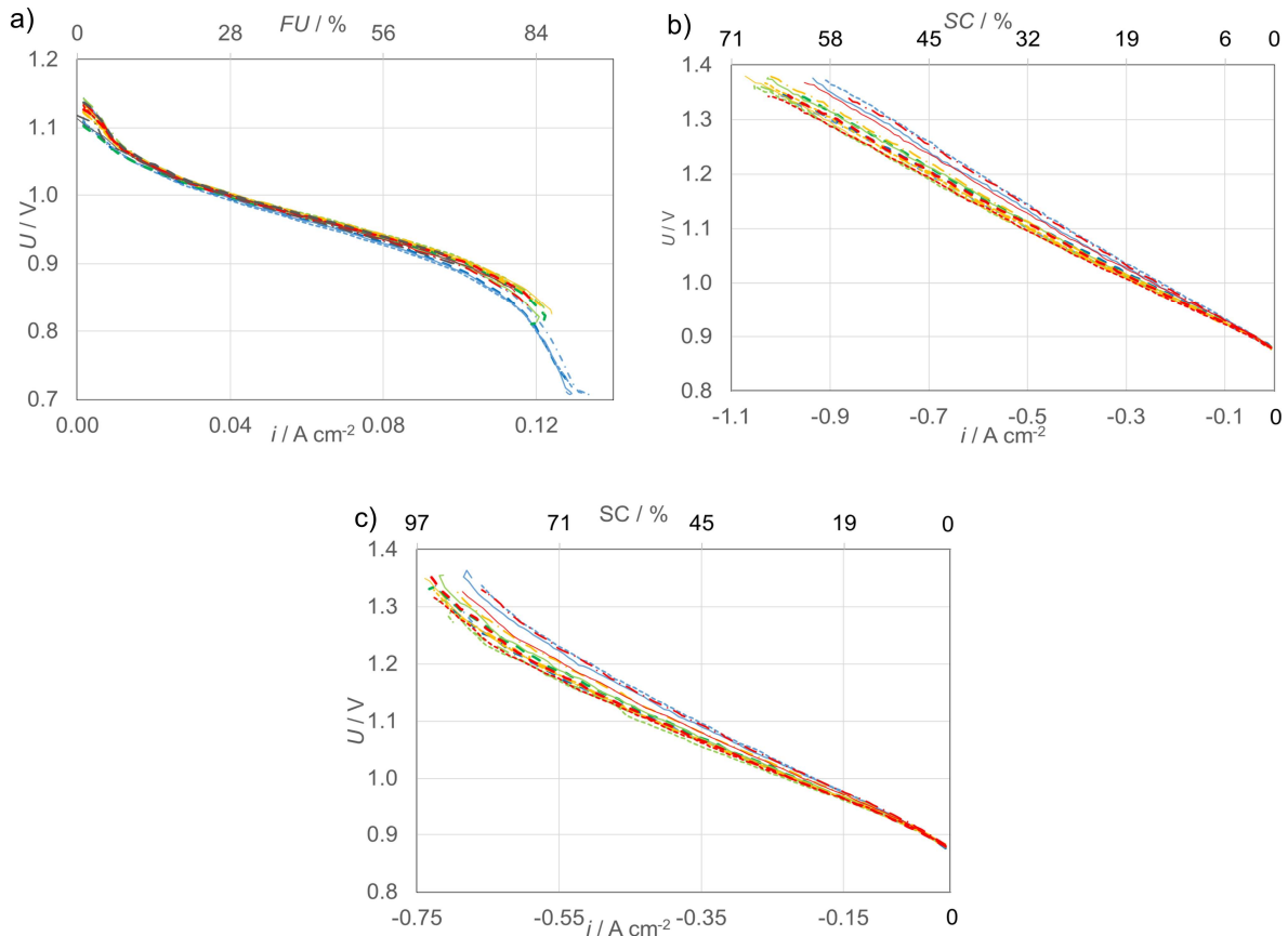
Figure 4: Acceptance iV curves of REFLEX stacks five batches of four stacks each, all performed at 700°C. Fig 4-a: stacks operated in SOFC mode. Flow rate of 1 NmL min -1 cm -2 of pure H 2 is provided to fuel electrode, air on the other side. Fig 4-b&c stacks operated in SOEC providing 90/10 vol.% H 2 O/H 2 mix to the fuel electrode, air on the other side, total fuel flow rate 12 and 6 NmL min -1 cm -2 respectively. For each curve, median cell voltage is reported for each stack, steam conversion is reported by secondary abscissa axis top of the graph. Color of the line identify manufacturing batches: blue for batch 0 delivered to Sylfen for in-lab tests of the SEH, green, yellow, red for batches 1, 2 and 3 to be implemented within REFLEX SEH modules, and finally black for spare batch 4.
