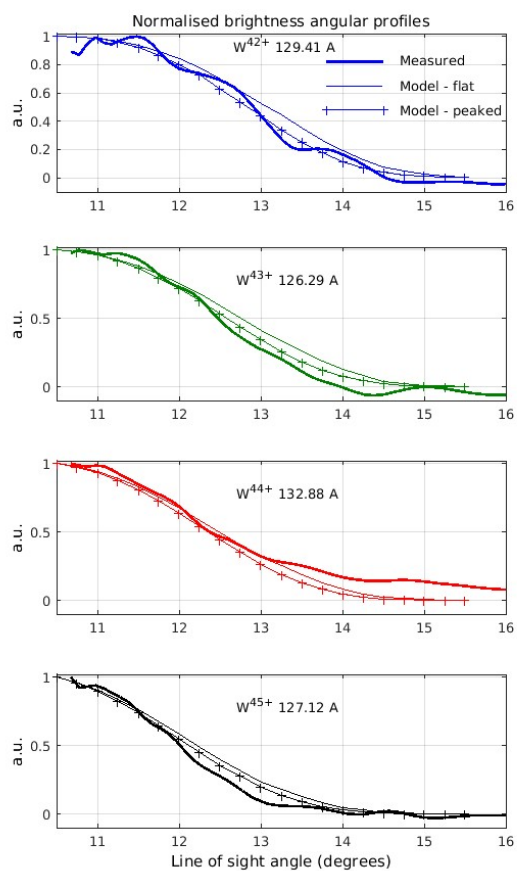
Figure 8: Angular profiles of the measured brightnesses (thick lines) and modelled brightness proxy (flat n_w profile: thin line, peaked n_w profile: thin line with +), all normalised to their maximum.
