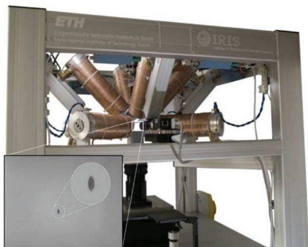
Figure 8. Experimental apparatus of the Octomag system, showing eight electromagnetic coils surrounding a workspace. Inset shows an optical image of an oval-shaped magnetic microrobot in the workspace. Adapted with permission. [85] Copyright 2009, IEEE.
