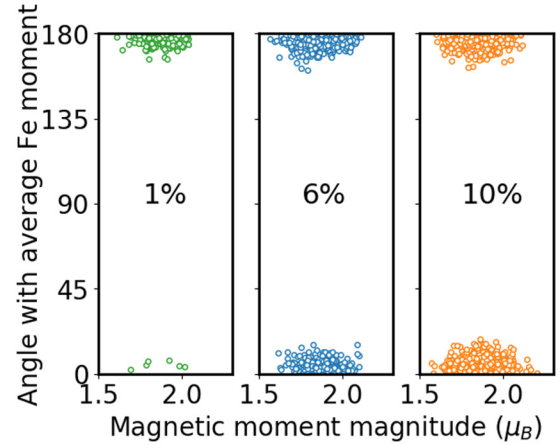
FIG. 7. Angle distribution between Mn magnetic moments and the average magnetic moment of Fe atoms, in random solutions at 1, 6, and 10 at. % Mn concentrations, using the KD model along with spin Monte Carlo simulations at 10 K.
