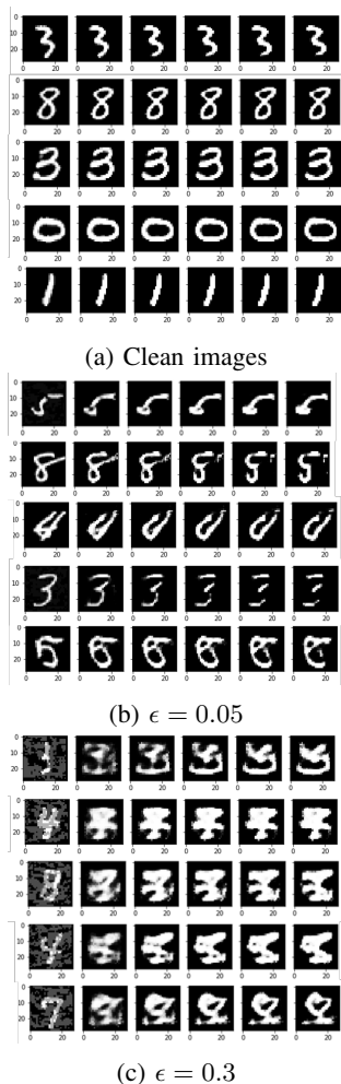
Fig. 1: Reverberations through a vanilla autoencoder of MNIST images and adversarial examples generated by attacking a LeNet model with FGSM attack. We can observe that while clean images remain stable during reverberation, adversarial images change. This is particularly the case when the perturbation size \epsilon is high. Measuring the difference between the original input and the output resulting from the fifth reverberation is enough to distinguish adversarial examples from clean images, as proved by the experiment presented below (see Section IV).
