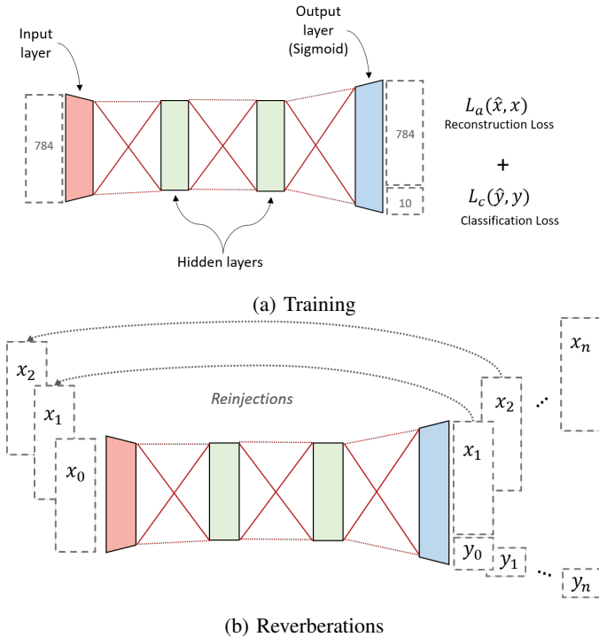
Fig. 3: Training and reverberations into a vanilla hybrid reverberant model for adversarial examples detection. The inputs are MNIST images (784 pixels, 10 classes). (a) The training is done by reducing the binary cross-entropy loss functions for reconstruction and classification. (b) Once the training is complete, the model can be used in detection mode. Each new incoming input is reverberated multiple times, and we measure the discrepancy between the logits and reconstructed images throughout the reverberation process.
