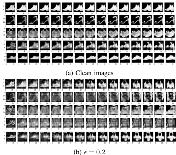
Fig. 2: Reverberations through a vanilla autoencoder of Fashion-MNIST images and adversarial examples generated by using the L_\infty -PGD attack. We can observe a phenomenon similar to the one observed in Figure 1 for MNIST images and adversarial examples generated with the FGSM attack.
