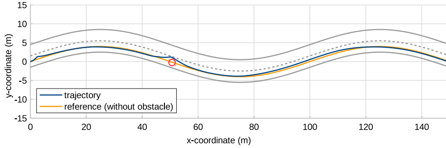
Fig. 8. Results of a co-simulation run.
