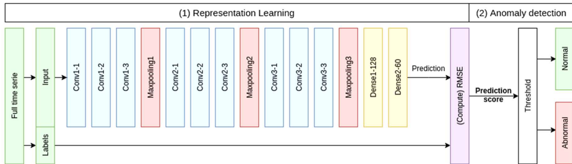
Fig. 2. Full anomaly detection pipeline. A 1D-CNN neural network is trained to predict the future of the time series. The RMSE between ground truth and predictio is compared to a threshold to define if a cell is abnormal.
