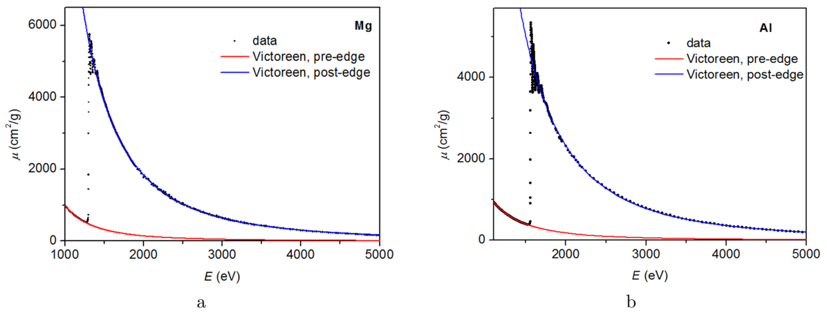
Figure 8: Victoreen trends below and above the K absorption edge in Mg (a) and Al (b).
