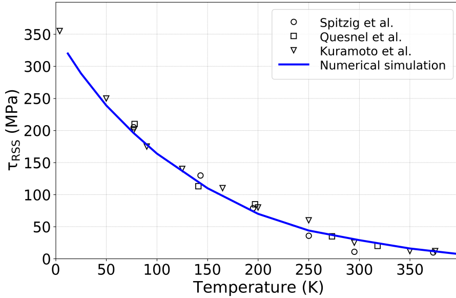
Figure 4: Validation of material model with experimental results reported by Spitzig et al. [38], Quesnel et al. [39] and Kuramoto et al. [40] against critical resolved shear stress.
