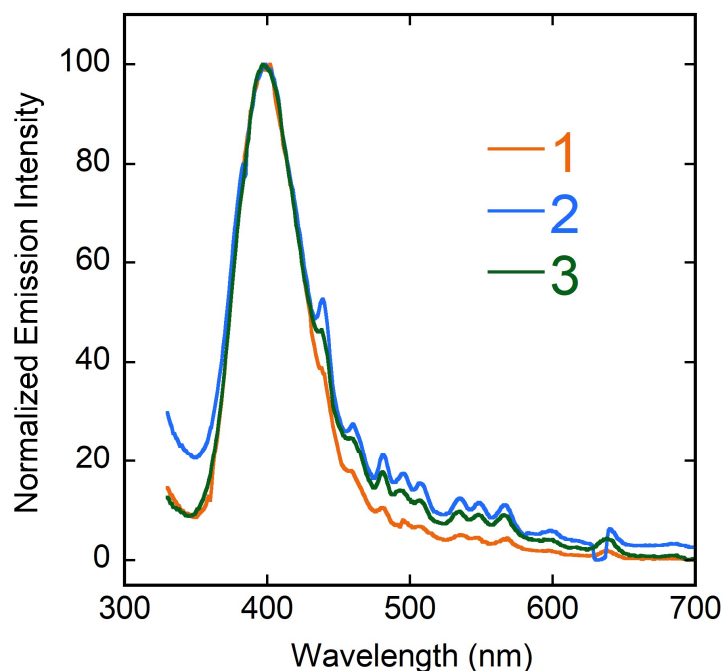
Fig. 6. Emission spectra of compounds 1–3 in the solid state at room temperature, under excitation at a wavelength of 260 nm.
