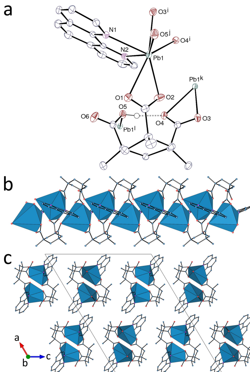
Fig. 4. (a) View of complex 3 . Displacement ellipsoids are drawn at the 50% probability level and carbon-bound hydrogen atoms are omitted. The hydrogen bond is shown as a dashed line. Symmetry codes: i = 1/2 - x, y + 1/2, 1/2 - z ; j = x, y + 1, z ; k = 1/2 - x, y - 1/2, 1/2 - z ; l = x, y - 1, z . (b) View of the monoperiodic helical polymer. (c) Packing with chains viewed end-on.
