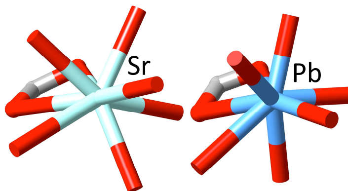
Fig. 3. Comparison, in similar orientations, of the donor atom arrays in (left) [\text{Sr}_3(\text{H}_3\text{kta})(\text{kta})_2] and (right) [\text{Pb}_3(\text{H}_3\text{kta})(\text{kta})_2] (stick representations, with the carbon atom of the chelating carboxylate also shown).
