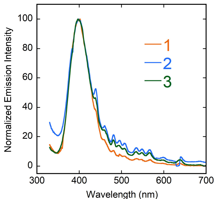
Fig. 6. Emission spectra of compounds 1–3 in the solid state at room temperature, under excitation at a wavelength of 260 nm.
