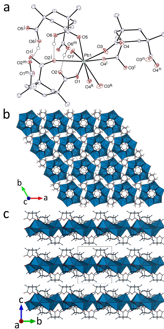
Fig. 2. (a) View of complex 2 . Displacement ellipsoids are drawn at the 50% probability level and carbon-bound hydrogen atoms are omitted. Hydrogen bonds are shown as dashed lines. Symmetry codes: i = y, y - x + 1, 1 - z ; j = 1 - y, x - y, z ; k = x - y + 1, x, 1 - z ; l = 2 - y, x - y + 1, z ; m = y - x + 1, 1 - x, z ; n = y - x + 1, 2 - x, z . (b) View of the dimeric polymer. (c) Packing with layers viewed edge-on.
