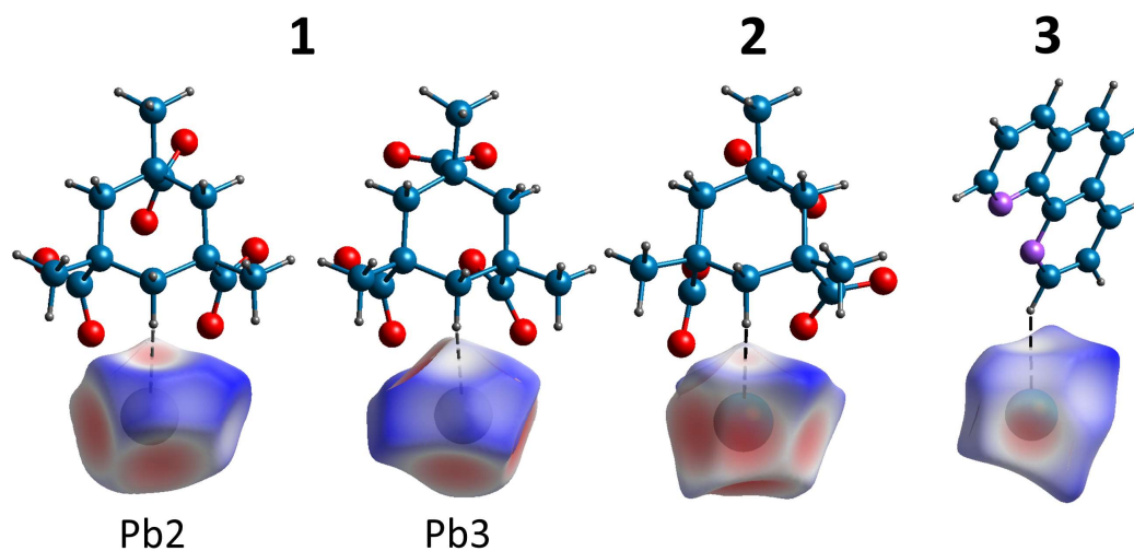
Fig. 5. HSs of the Pb II cations mapped with d_{\text{norm}} showing the possible Pb II ···H interactions. The larger red dots on the HS correspond to the location of chlorine, oxygen or nitrogen donors.
