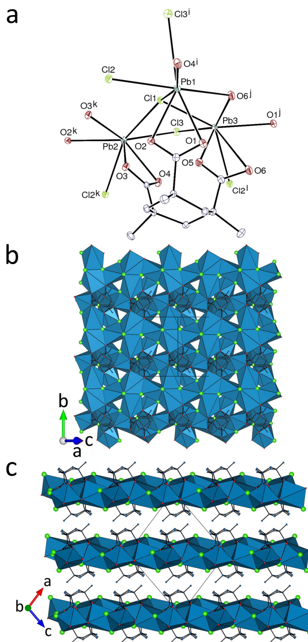
Fig. 1. (a) View of complex 1 . Displacement ellipsoids are drawn at the 50% probability level and hydrogen atoms are omitted. The longest Pb–Cl contact is not shown. Symmetry codes: i = x - 1/2, 1/2 - y, z - 1/2 ; j = 1 - x, 1 - y, 1 - z ; k = 1 - x, -y, 1 - z ; l = x + 1/2, 1/2 - y, z + 1/2 . (b) View of the diperiodic polymer with lead(II) coordination polyhedra colored blue. (c) Packing with layers viewed edge-on.
