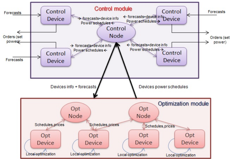
Fig. 2. SMARTERCtrl optimization and control modules, interactions
