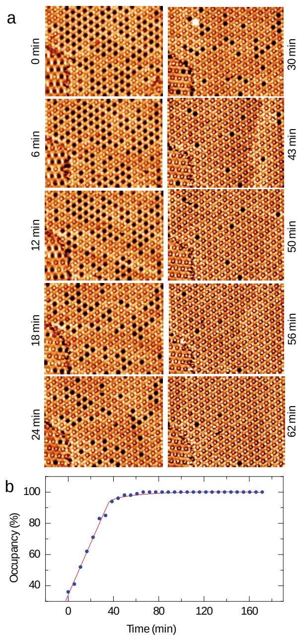
Figure 6. (a) Sequential STM images of the ZnPc adsorption into the organic host nanoarchitecture, 75 \times 55 nm 2 ; V_s = 0.6 V, I_t = 400 pA. (b) Evolution of the cavity occupancy of the host nanoarchitecture (percentage) with time (min). The red curve is a fit of the occupancy behavior.
