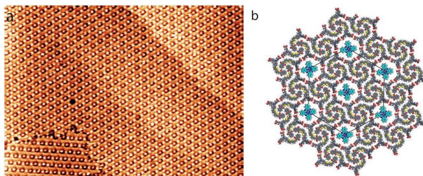
Figure 7. (a) STM image ZnPc-dye assembly after one hour, 120 \times 85 \text{ nm}^2 , V_s = 0.6 \text{ V} , I_t = 400 \text{ pA} . (b) Model of the ZnPc-dye guest–host structure.
