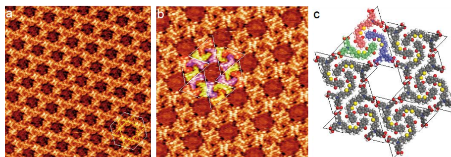
Figure 2. STM images of the self-assembly of compound-1 into a Kagomé nanoarchitecture with hexagonal cavities on graphite, (a) 38 \times 38 nm 2 ; (b) 20 \times 20 nm 2 ; V_s = 0.6 V, I_t = 450 pA. As a guide for the eyes, the hexagonal unit cell (white solid lines) and the Kagomé star (yellow solid lines) have been superimposed onto the STM image in (a). (c) Model of the Kagomé nanoarchitecture observed in (a,b). As a guide for the eyes, dashed white and black triangles highlighting triangular trimers have been superimposed onto the STM image in (b) and the model in (c), respectively.
