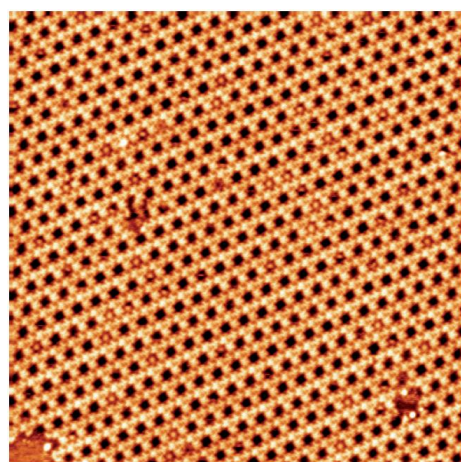
Figure 3. STM image of the dye Kagomé network after coronene deposition, 56 \times 56 \text{ nm}^2 ; V_s = 0.6 \text{ V} , I_t = 400 \text{ pA} .
