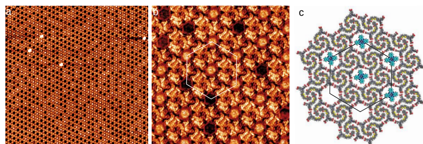
Figure 5. STM images of the organic layer after subsequent deposition of ZnPc with a low concentration ( 2.0 \times 10^{-6} M), (a) 135 \times 135 nm 2 , (b) 20 \times 20 nm 2 ; V_s = 0.6 V, I_t = 400 pA. (c) Model of the guest–host structure corresponding to the area with the superimposed white hexagon highlighted in (b).
