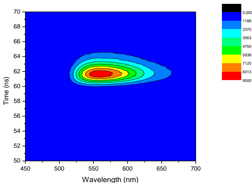
Figure 4 Time-Resolved Emission Spectroscopy of 0.03 wt% 4-dimethylamino-4'-nitrostilbene in toluene, quenched with 5 wt% of Hünig's base. \tau_{\text{mean}} = 1.50 \text{ ns} ( \lambda_{\text{ex}} = 368 \text{ nm} )
