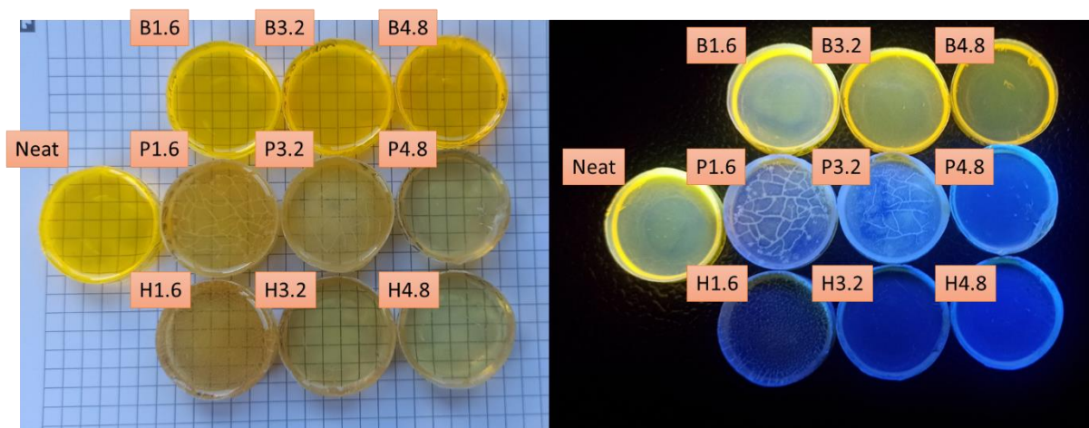
Figure 5 Scintillators composed of polystyrene containing p -terphenyl, DANS and quenchers, under visible light (left) and 368 nm UV (right), pictured 18 months after preparation. B, P and H stand for Benzophenone, Piperidine and Hünig's base, respectively with their added concentration.
