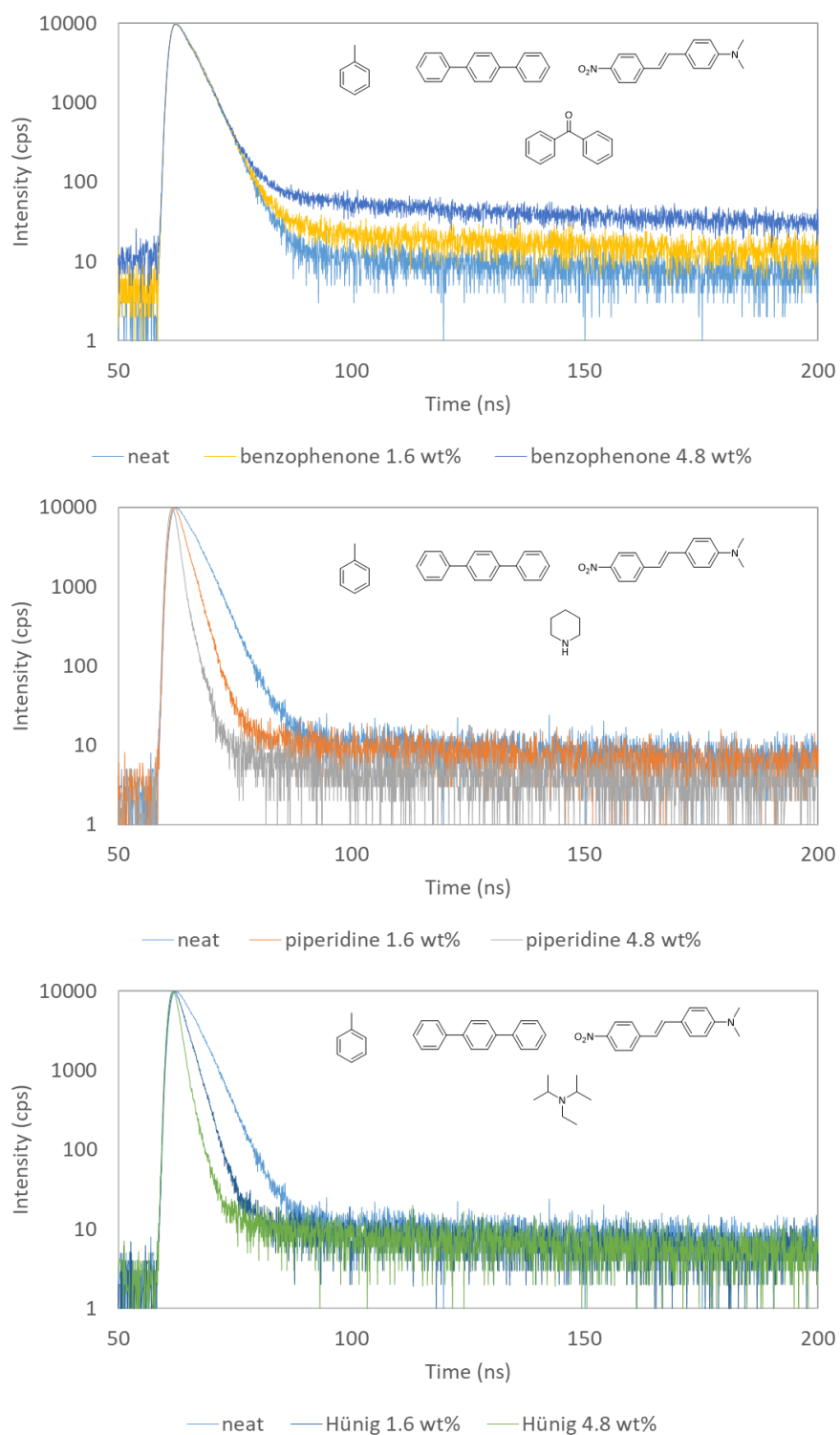
Figure 3 Photoluminescence quenching of a plastic scintillator composed of PS + p-terphenyl 1.5 wt% + DANS 0.01 wt% with different amounts of benzophenone (top), piperidine (middle) or Hünig's base (bottom). The same unquenched, reference material is added on each figure ( \tau_{ex} = 274 \text{ nm} ; \tau_{obs} = 560 \text{ nm} ).
