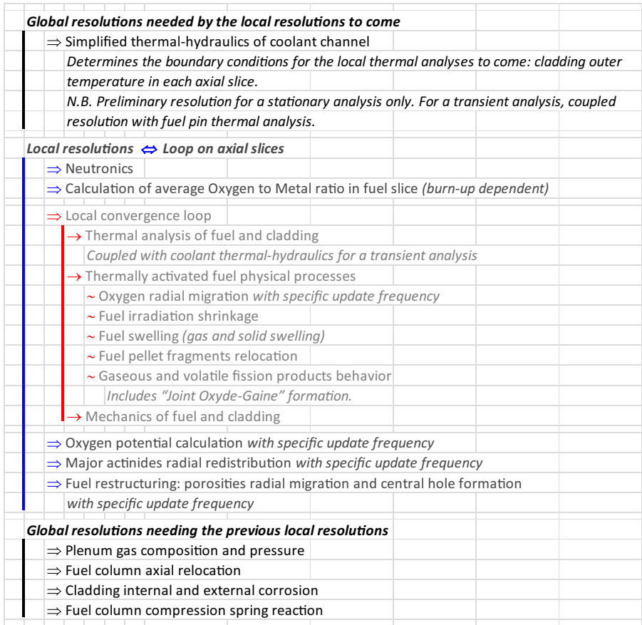
FIGURE 9.15 GERMINAL multiphysics computational scheme for one step [7].
