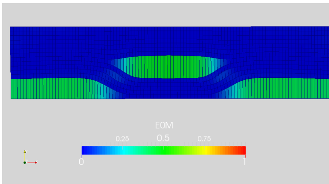
b) Damage extension (strain loading 0.13%) (mesh size=t/100)
