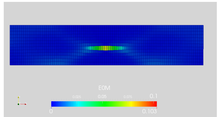
d) Damage extension (strain loading 0.06%) (mesh size=t/100)
