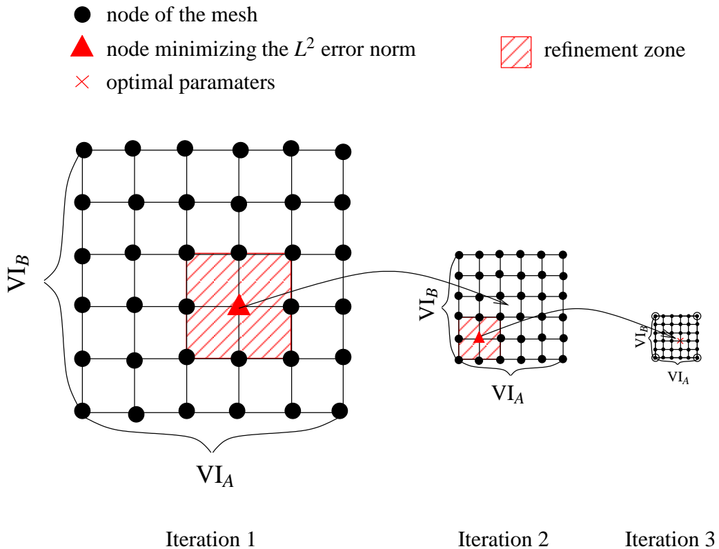
Figure 1: Refinement procedure to determine optimal individual diffusion coefficients (obtained here within 3 iterations).
