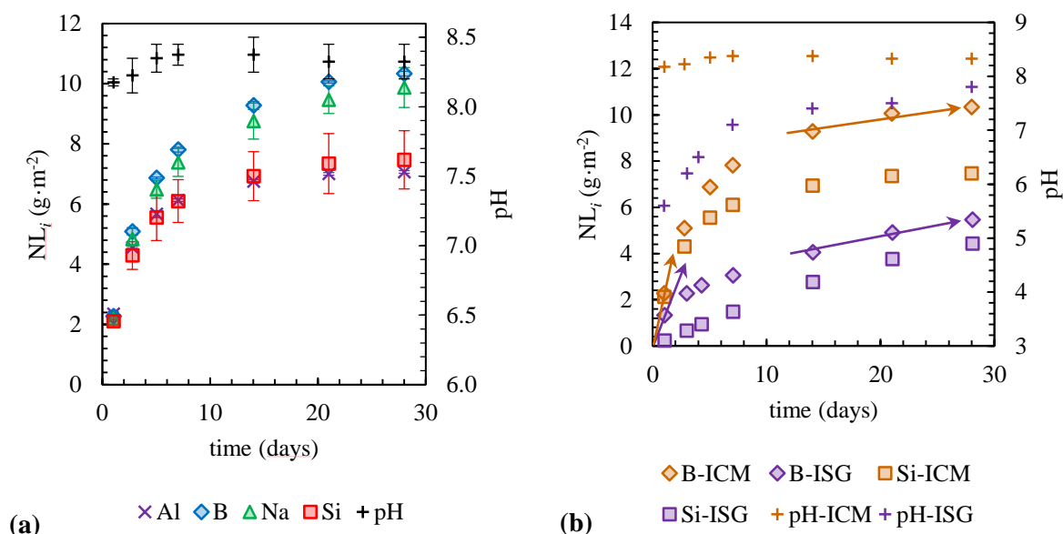
Figure 6. (a) Evolution of NL and pH during wastefrom leaching (error bars represent the data dispersion between the duplicates). (b) Compared evolution of NL and pH during the leaching of ISG and In-Can-produced wastefrom. The arrows are a visual guide to estimate the drop in alteration rate.
