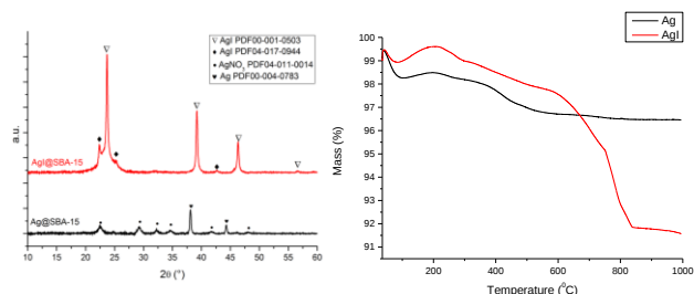
Figure 2: Left; XRD of Ag@SBA-15 (black) and AgI@SBA-15 (red). Note the presence of both Ag and AgNO 3 in the Ag@SBA-15 samples. Only AgI is detected after I 2 addition. Right; TGA of Ag@SBA-15 (black) and AgI@SBA-15 (red). Mass increase at 200 °C is ascribed to Ag 2 O formation. However it starts to decompose almost immediately after formation. 17,28 Mass loss beginning at 380 °C in the Ag@SBA-15 samples is believed to be AgNO 3 decomposition. Mass loss beginning at 600 °C in the AgI@SBA-15 samples is believed to be AgI decomposition.
