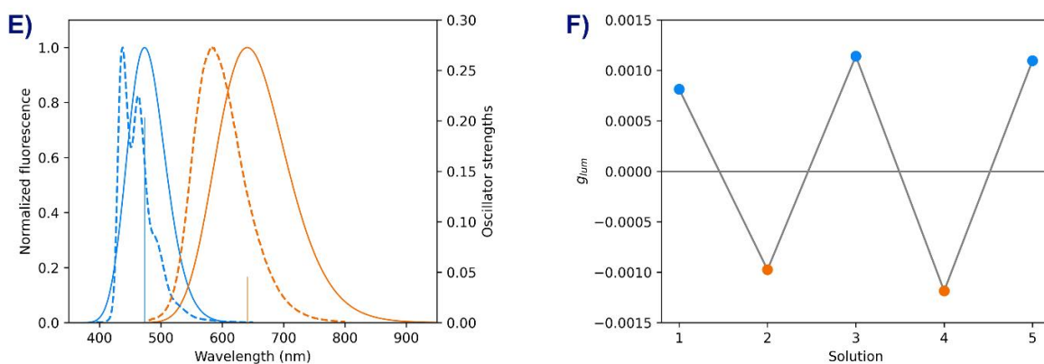
Figure 4: Experimental and computational spectra of C-29 (blue) and C-29•H + (orange). A) and B) Experimental absorption spectra (color) recorded in \text{CH}_2\text{Cl}_2 ( C = 5 \times 10^{-5} M), along with oscillator strengths for selected transitions (grey bars) and full predicted spectra (black curves) from TD-DFT calculations. NBOs for the HOMO and LUMO of each compound are shown as inset. C) and D) Experimental circular dichroism (CD) spectra for the (+)-enantiomer (full color) and (-)-enantiomer (dashed color) recorded in \text{CH}_2\text{Cl}_2 ( C = 5 \times 10^{-6} M), along with rotatory strengths for selected transitions (grey bars) and full predicted spectra (black curves) from TD-DFT calculations. E) Experimental emission spectra (dashed curves) recorded in \text{CH}_2\text{Cl}_2 ( C = 5 \times 10^{-5} M), along oscillator strength for S_1 \rightarrow S_0 transition (bars) and predicted spectra (full curves) from TD-DFT calculations. F) Switch of g_{lum} value for (+)- C-29 . 1: initial solution ( C = 5 \times 10^{-5} M in \text{CH}_2\text{Cl}_2 ) 2 and 4: after protonation by addition of 4 mmol of TFA; 3 and 5: after addition of 4 mmol of DBU.
