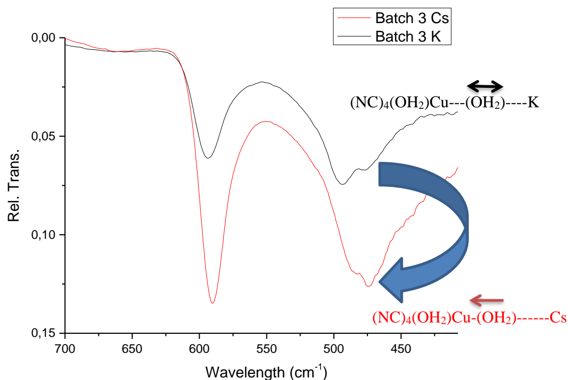
Figure 11: FT-IR of batch 3 before (black) and after (red) Cs/K exchange. Note the inversion of the relative strength of the \nu(\text{Cu-N}) stretches.
