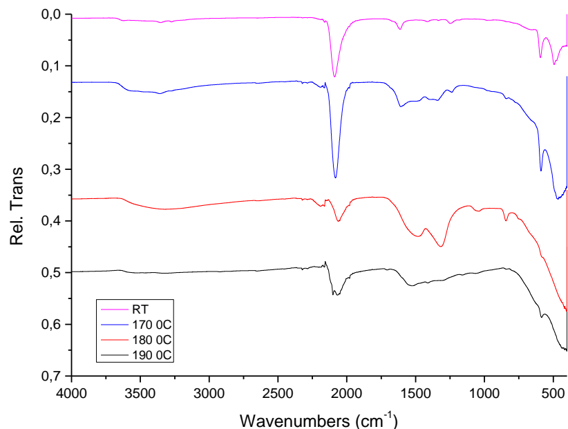
Figure 8: FT-IR of batch 3 at room temperature, as well as after various heat treatments from 170 °C to 250 °C..
