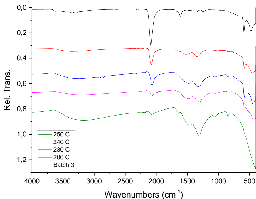
Figure 10: FT-IR of Cs exchanged batch 3 taken before thermal treatment began (black) and after thermal treatment at 200, 230, 240 and 250°C.
