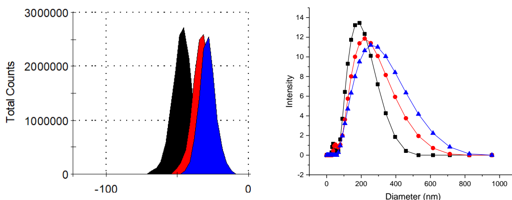
Figure 4: Zeta Potential (left) and size (right) measurements of each batch measured in mV and nm respectively.
