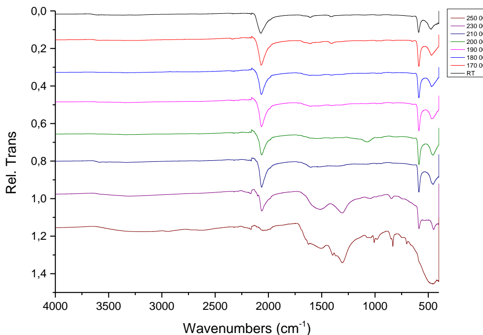
Figure 7: FT-IR of batch 2 at room temperature, as well as after various heat treatments from 170 °C to 250 °C. Each scan corresponds to 4 hours at that temperature. The sample is the same one throughout the experiment.
