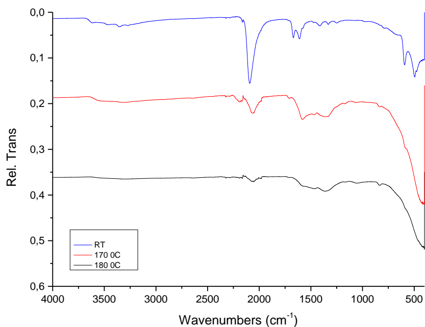
Figure 9: FT-IR of batch 4 at room T (blue) and after heating at 170 °C (red) and 180 °C (black). the \nu(\text{CN}) stretch has decreased in strength by 75 %.
