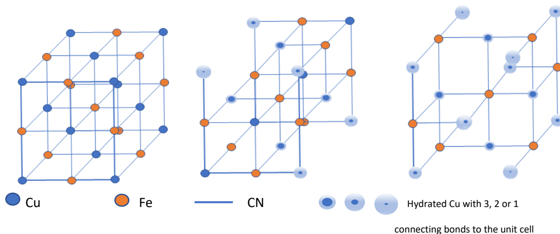
Figure 5: From left to right Cu-HCF with 0, 20, and 50 % of the Fe(CN) 6 4- sites vacant. As the number of vacancies increase the materials dependence on water to complete the structure increases.
