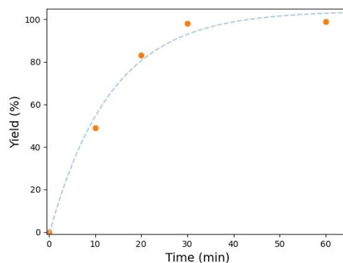
Figure 1. 1 H NMR monitoring of the formation of pinBO(CH 2 ) 6 OBpin as a function of time.
