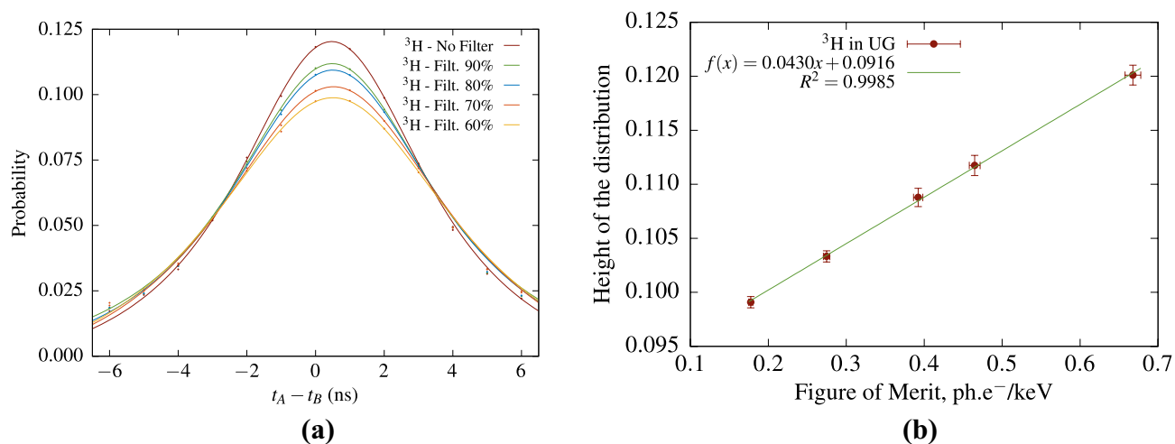
Figure 7. Cross-correlation studies with ^3\text{H} in Ultima Gold cocktail and various levels of grey filters. The cross-correlation spectra (a) are fitted within \pm 3 ns with a Voigt profile in order to evaluate the height of the distribution.
