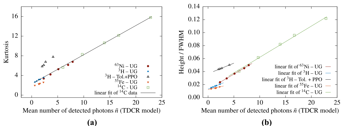
Figure 6. Kurtosis of the cross-correlation spectra—the data points are measurement results and the linear fit is performed on the ^{14}\text{C} data and extrapolated (a). The average number of detected photons is calculated from the TDCR model. (b) Scaling the cross-correlation data H_0/\text{FWHM} vs \bar{n} . The data points are from measurements of various LS-sources and the average number of photons is calculated from the TDCR model.
