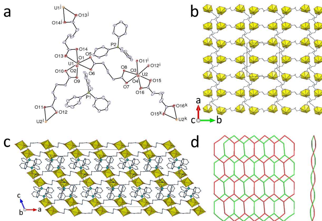
Figure 8. (a) View of compound 8 . Displacement ellipsoids are drawn at the 50% probability level. Solvent molecules and hydrogen atoms are omitted. Only one position of the disordered parts is represented. Symmetry codes: i = x - 1, y, z ; j = 1 - x, -y, 1 - z ; k = -x, 2 - y, 1 - z ; l = x + 1, y, z . (b) View of the twofold interpenetrated diperiodic networks. (c) Packing with sheets viewed edge-on. (d) Simplified view of the twofold interpenetration of diperiodic networks down [001] (left) or [100] (right).
