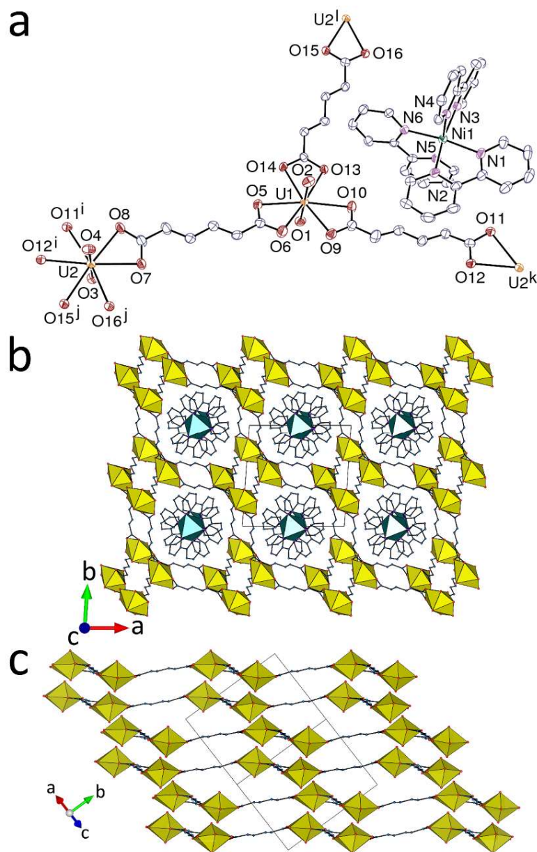
Figure 2. (a) View of compound 2. Displacement ellipsoids are drawn at the 50% probability level. Solvent molecules and hydrogen atoms are omitted. Symmetry codes: i = x, y - 1, z - 1 ; j = x - 1, y, z - 1 ; k = x, y + 1, z + 1 ; l = x + 1, y, z + 1 . (b) and (c) Packing with sheets viewed obliquely or edge-on, respectively; counterions are omitted in (c) for clarity.
