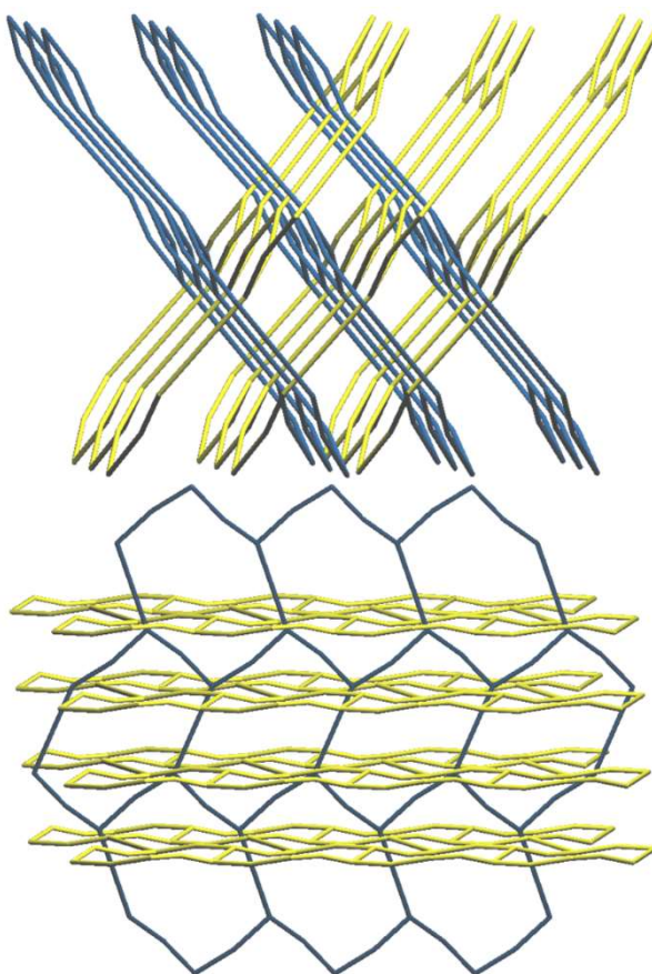
Figure 10. Two views of the simplified representation of the twofold polycatenation of diperiodic networks in complex 9 , slightly rotated from the zone direction (top), and showing the double crossing of each hexagonal ring (bottom).
