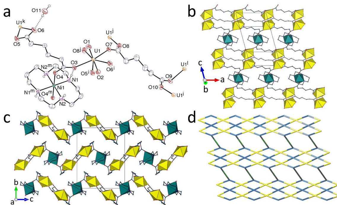
Figure 3. (a) View of compound 3 . Displacement ellipsoids are drawn at the 30% probability level. Carbon-bound hydrogen atoms are omitted and hydrogen bonds are shown as dashed lines. Only one position of the disordered dicarboxylate ligand is shown. Symmetry codes: i = x + 1, y, z ; j = 2 - x, 1 - y, 2 - z ; k = x - 1, y, z ; l = 3 - x, 1 - y, 2 - z ; m = 1 - x, 1 - y, 1 - z . (b) View of the diperiodic coordination polymer with uranium coordination polyhedra yellow and those of nickel green. (c) Packing with sheets viewed edge-on. (d) Nodal representation of the network (uranium nodes, yellow; nickel links, green; dicarboxylate nodes, dark blue; same orientation as in part b).
