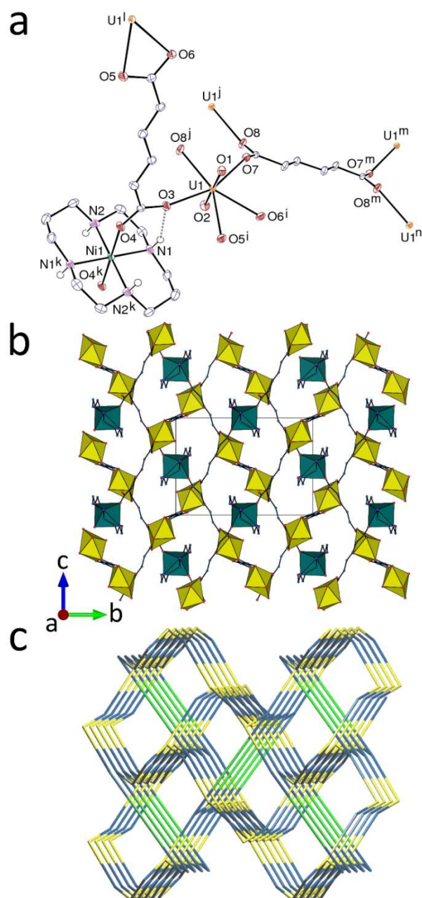
Figure 4. (a) View of compound 4. Displacement ellipsoids are drawn at the 50% probability level. Solvent molecules and carbon-bound hydrogen atoms are omitted, and the hydrogen bond is shown as a dashed line. Symmetry codes: i = x - 1/2, 1/2 - y, z + 1/2 ; j = 1 - x, 1 - y, 1 - z ; k = 2 - x, 1 - y, 2 - z ; l = x + 1/2, 1/2 - y, z - 1/2 ; m = -x, 1 - y, 1 - z ; n = x - 1, y, z . (b) View of the triperiodic framework with uranium coordination polyhedra yellow and those of nickel green. (c) Nodal representation of the framework (uranium nodes, yellow; nickel links, green; dicarboxylate nodes, dark blue; orientation slightly rotated with respect to that in part b).
