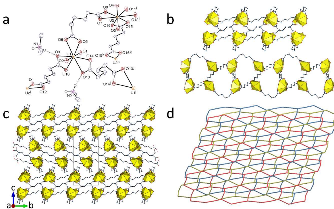
Figure 6. (a) View of compound 6 . Displacement ellipsoids are drawn at the 50% probability level. Carbon-bound hydrogen atoms are omitted and hydrogen bonds are shown as dashed lines. Symmetry codes: i = x + 1, y - 1, z ; j = 1 - x, -y, 1 - z ; k = 2 - x, 2 - y, 1 - z ; l = x - 1, y + 1, z . (b) Two views of the threefold interpenetrated diperiodic networks down [100] (top) or [010] (bottom). (c) Packing with sheets viewed edge-on and counterions omitted. (d) Simplified view of the threefold interpenetration of diperiodic networks down [001] .
