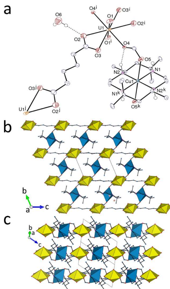
Figure 5. (a) View of compound 5 . Displacement ellipsoids are drawn at the 50% probability level. Carbon-bound hydrogen atoms are omitted and hydrogen bonds are shown as dashed lines. Symmetry codes: i = 1 - x, -y, -z ; j = 2 - x, -y, 1 - z ; k = 1 - x, 1 - y, 1 - z . (b) View of the dimeric coordination polymer with uranium coordination polyhedra yellow and those of copper blue. (c) Packing with sheets viewed edge-on.
