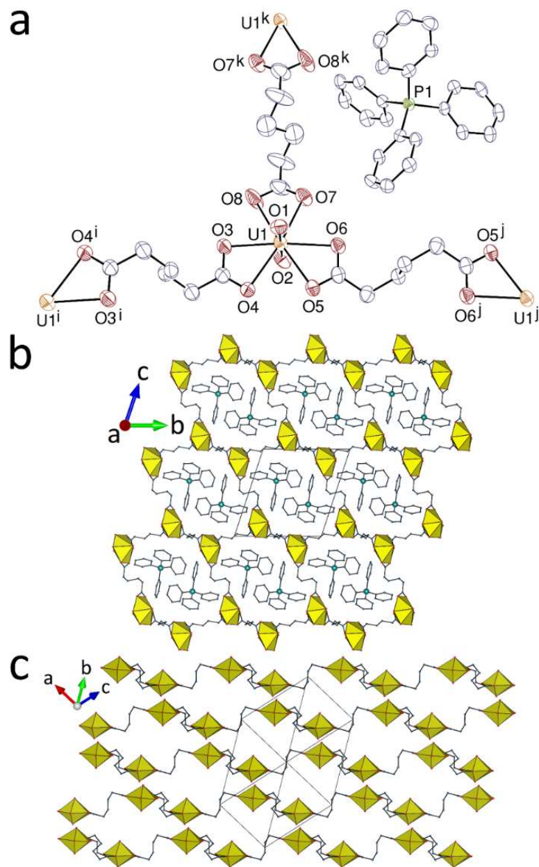
Figure 1. (a) View of compound 1 . Displacement ellipsoids are drawn at the 50% probability level and hydrogen atoms are omitted. Symmetry codes: i = -x, 2 - y, 2 - z ; j = 2 - x, 1 - y, 2 - z ; k = 1 - x, 2 - y, 1 - z . (b) View of the diperiodic polymer with uranium coordination polyhedra colored yellow. (c) Packing with sheets viewed edge-on and counterions omitted for clarity.
