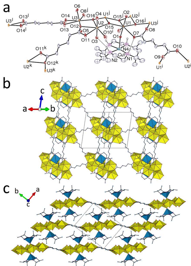
Figure 7. (a) View of compound 7. Displacement ellipsoids are drawn at the 30% probability level. Carbon-bound hydrogen atoms are omitted and hydrogen bonds are shown as dashed lines. Symmetry codes: i = 1 - x, 1 - y, -z ; j = 1 - x, 1 - y, 1 - z ; k = 2 - x, -y, 1 - z ; l = 2 - x, -y, 2 - z . (b) View of the diperiodic coordination polymer with uranium coordination polyhedra yellow and those of copper blue. (c) Packing with sheets viewed edge-on.
