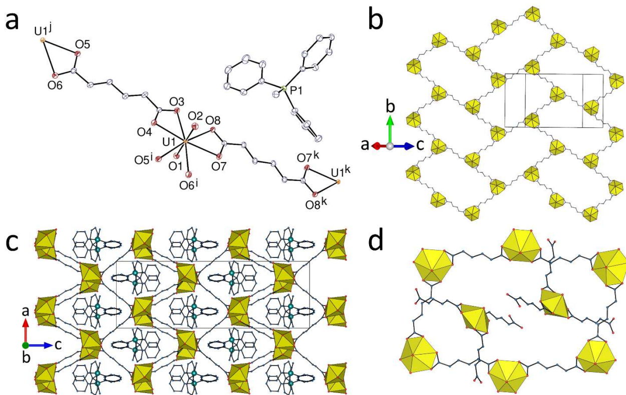
Figure 9. (a) View of compound 9 . Displacement ellipsoids are drawn at the 50% probability level. Solvent molecules and hydrogen atoms are omitted. Symmetry codes: i = 1 - x, y - 1/2, 1/2 - z ; j = 1 - x, y + 1/2, 1/2 - z ; k = 2 - x, -y, 1 - z . (b) View of the hcb diperiodic network. (c) View of the polycatenated structure with sheets edge-on. (d) View of one hexanuclear ring with the two included uranyl cations pertaining to the two intersecting planes.
