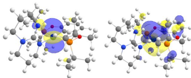
Figure 3. HOMO-1 (left) and LUMO (right) of 7
