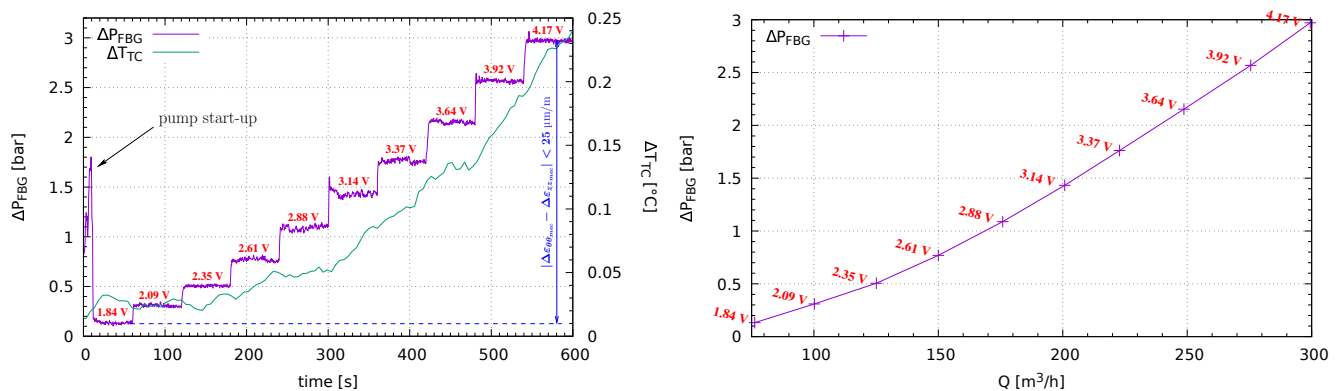
Figure 10. Air flow rate steps & corresponding FBG non-intrusive pressure variation measurement vs. time (left) and non-intrusive pressure variation vs. air flow rate measurements (right) on Mercure facility.
